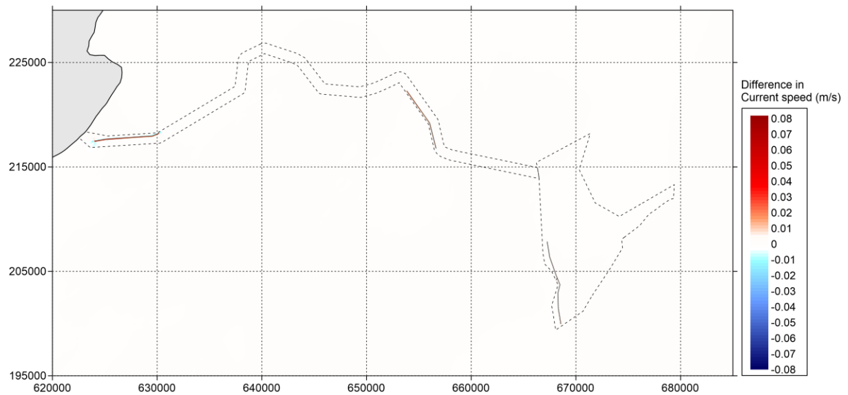
Figure 5.93 Difference in current speed (in metres/second) between 'Baseline' and 'Additional Layout' during neap tide (positive means increase of current speed by option and vice versa) – peak flood
