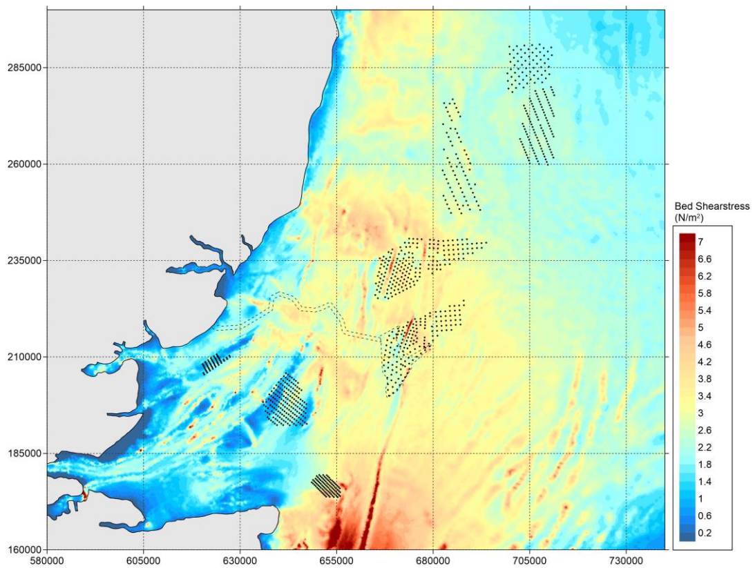
Figure 5.49 All windfarms ('Cumulative') – Bed shear stress during spring tide - peak flood.
