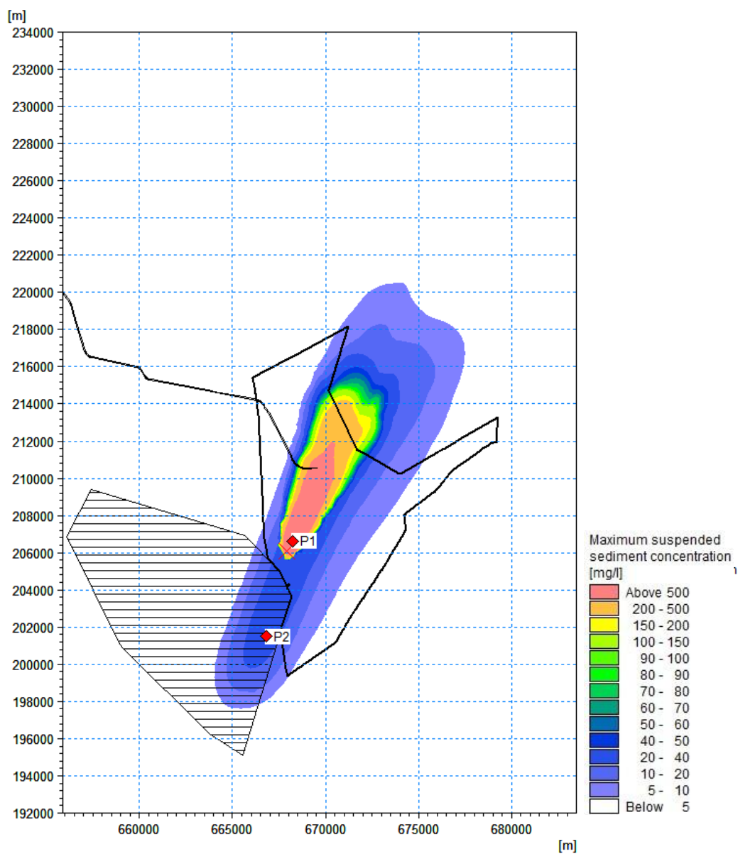
Figure 7.122 Maximum suspended sediment concentration during array disposal occurring near the seabed – Peak ebb during spring tide ('Zone 1 & 3' material) (red point = time series extraction point)
