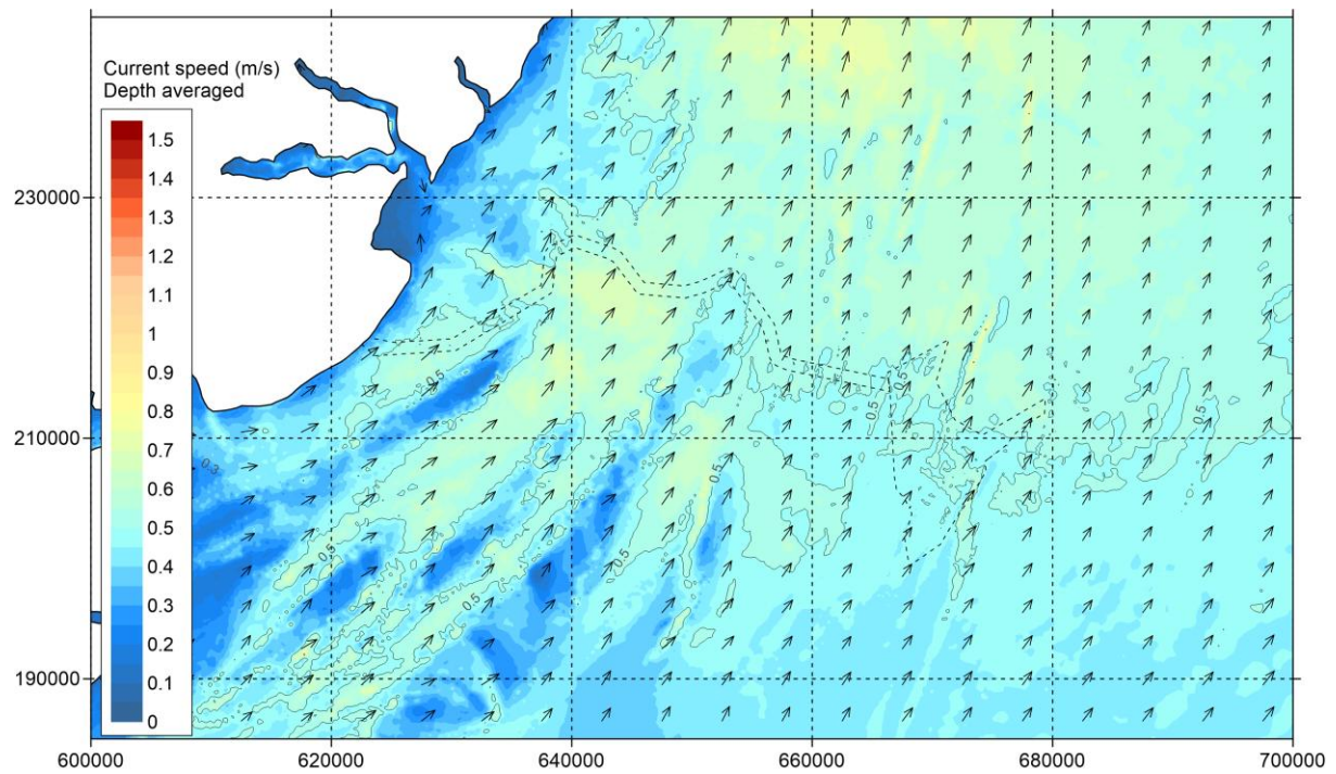
Figure 5.27 Baseline - Current speed during neap tide - peak ebb (zoomed in).
