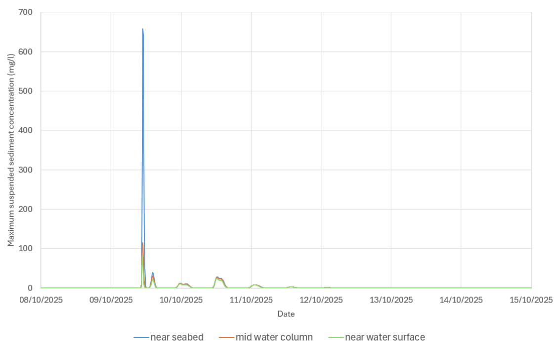
Figure 7.126 Time series of suspended sediment concentration at P2 during sediment disposal near seabed, middle of water column and near water surface – Peak ebb during spring tide ('Zone 1 & 3' material)
