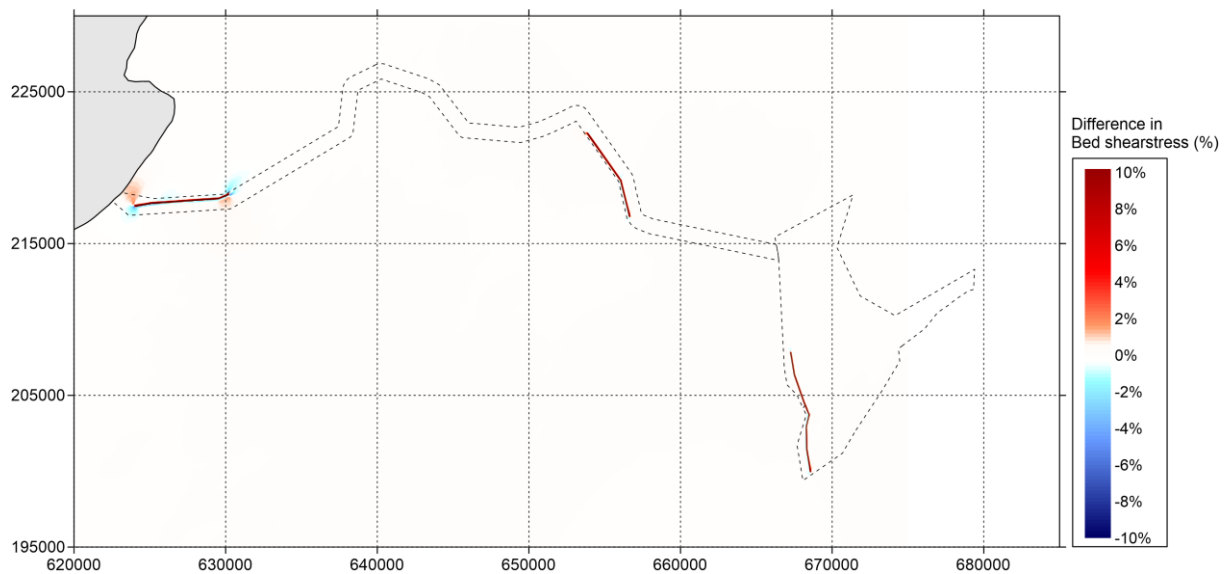
Figure 5.100 Difference in bed shear stress (in percent) between 'Baseline' and 'Additional Layout' during spring tide (positive means increase of bed shear stress by option and vice versa) – peak ebb.
