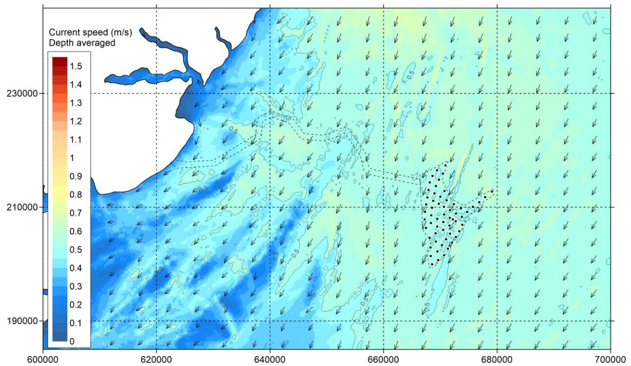
Figure 5.31 Option - Current speed during neap tide - peak flood.
