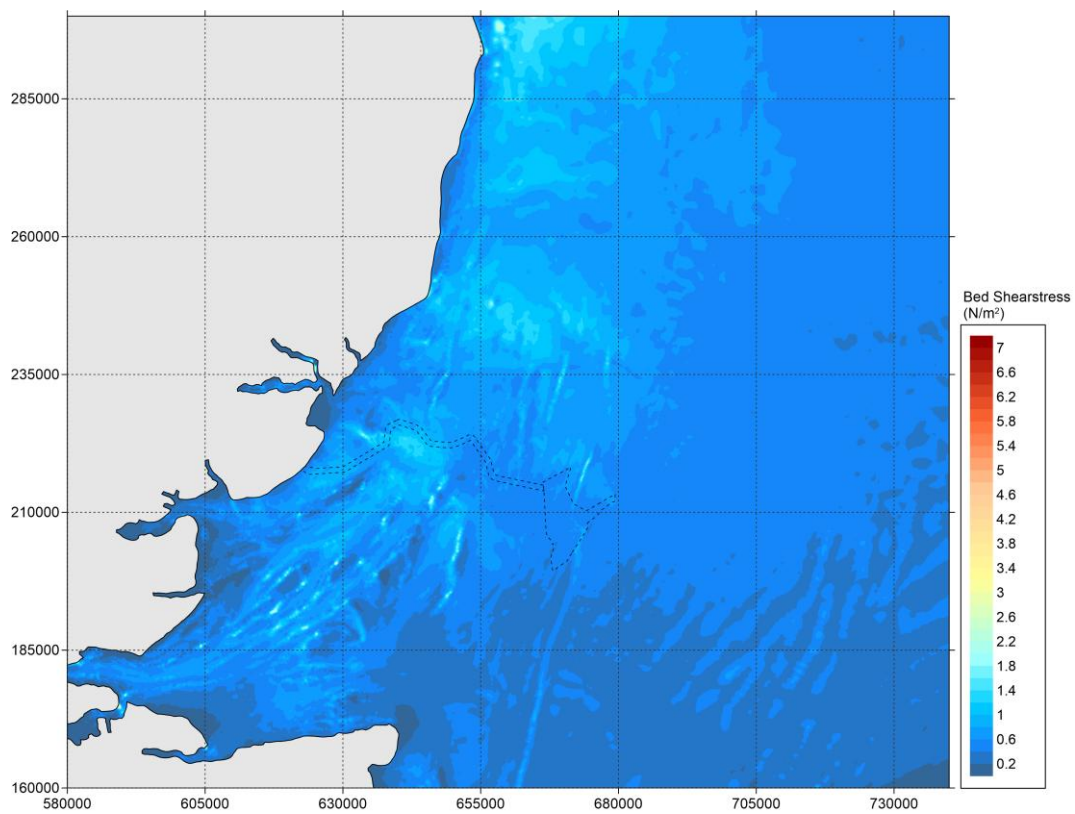
Figure 5.44 Baseline – Bed shear stress during neap tide - peak ebb (zoomed out).
