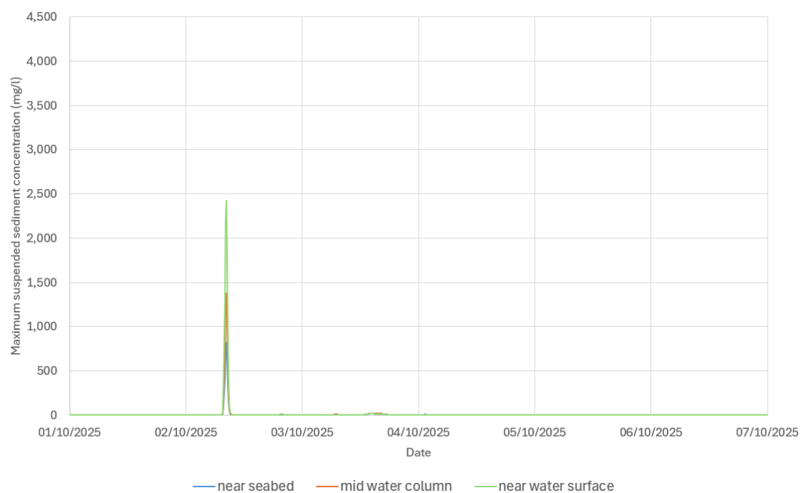
Figure 7.108 Time series of suspended sediment concentration at P1 during sediment disposal near seabed, middle of water column and near water surface - Slack water near high water during neap tide ('Zone 1 & 3' material)
