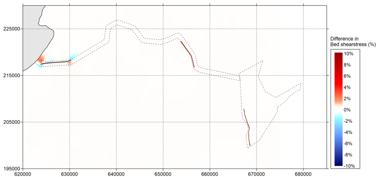
Figure 5.104 Difference in bed shear stress (in percent) between 'Baseline' and 'Additional Layout' during neap tide (positive means increase of bed shear stress by option and vice versa) – peak ebb.
