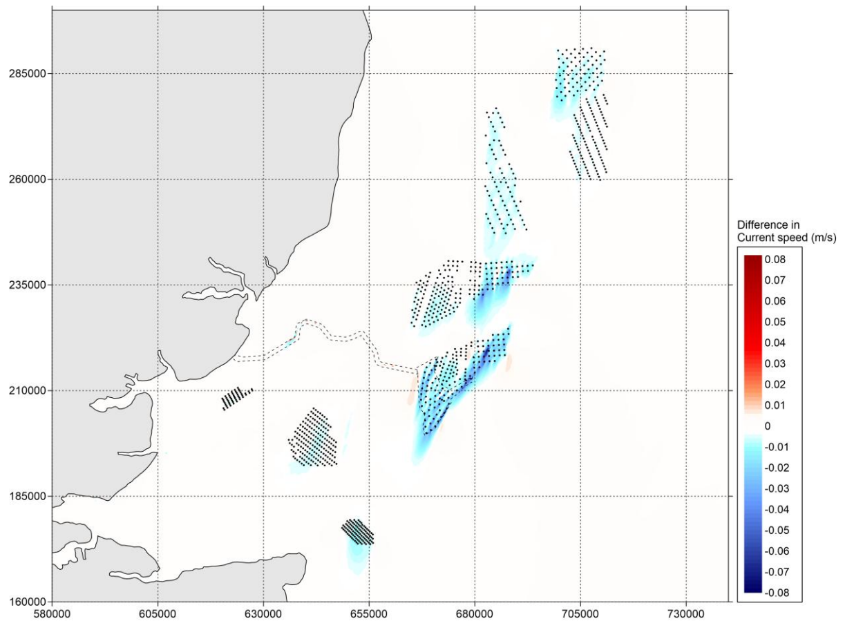
Figure 5.73 Difference in current speed (in metres/second) between 'Baseline' and 'Cumulative' during spring tide (positive means increase of current speed by option and vice versa) – peak flood
