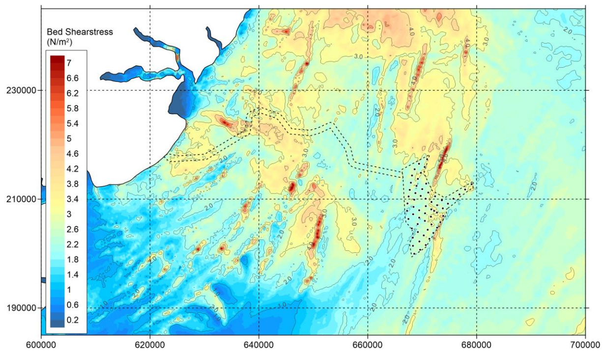
Figure 5.46 Option – Bed shear stress during spring tide - peak ebb.
