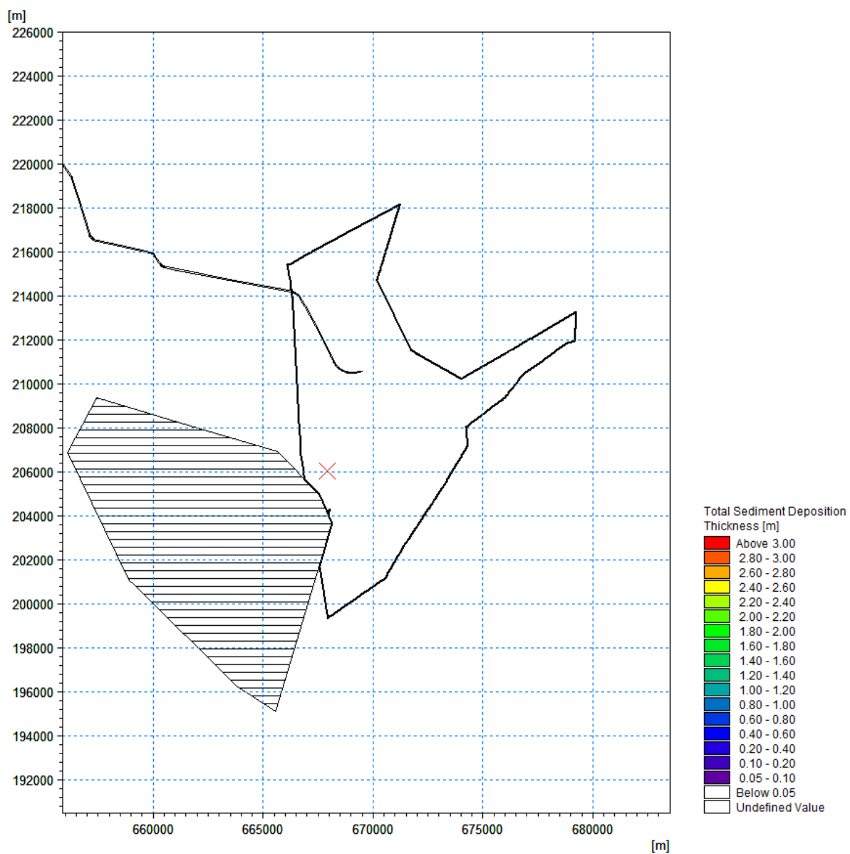
Figure 7.121 Total deposition thickness during sediment disposal - Peak flood during spring tide ('Zone 1 & 3' material)
