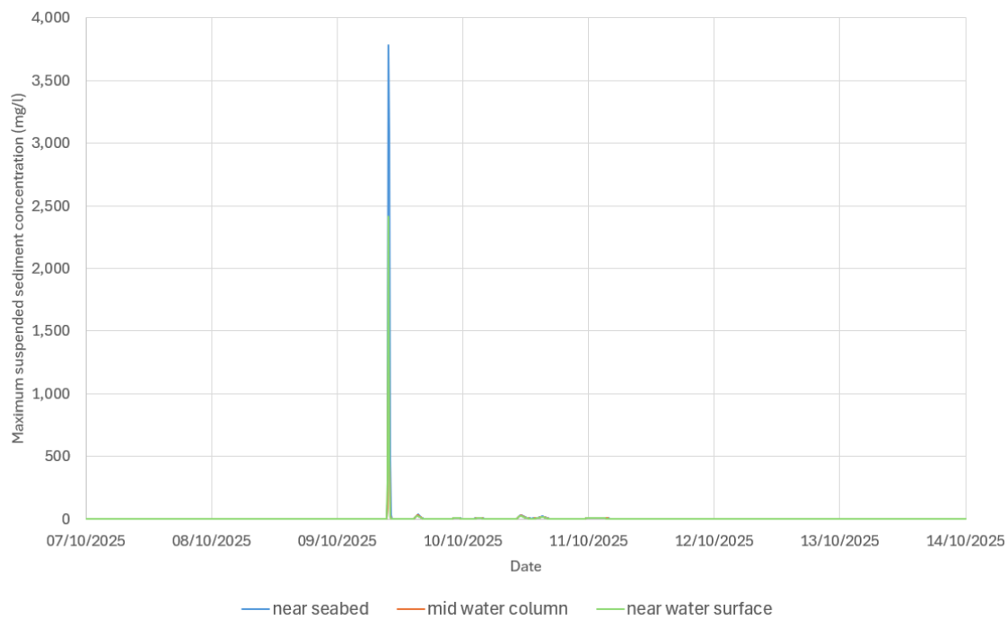
Figure 7.119 Time series of suspended sediment concentration at P1 during sediment disposal near seabed, middle of water column and near water surface – Peak flood during spring tide ('Zone 1 & 3' material)
