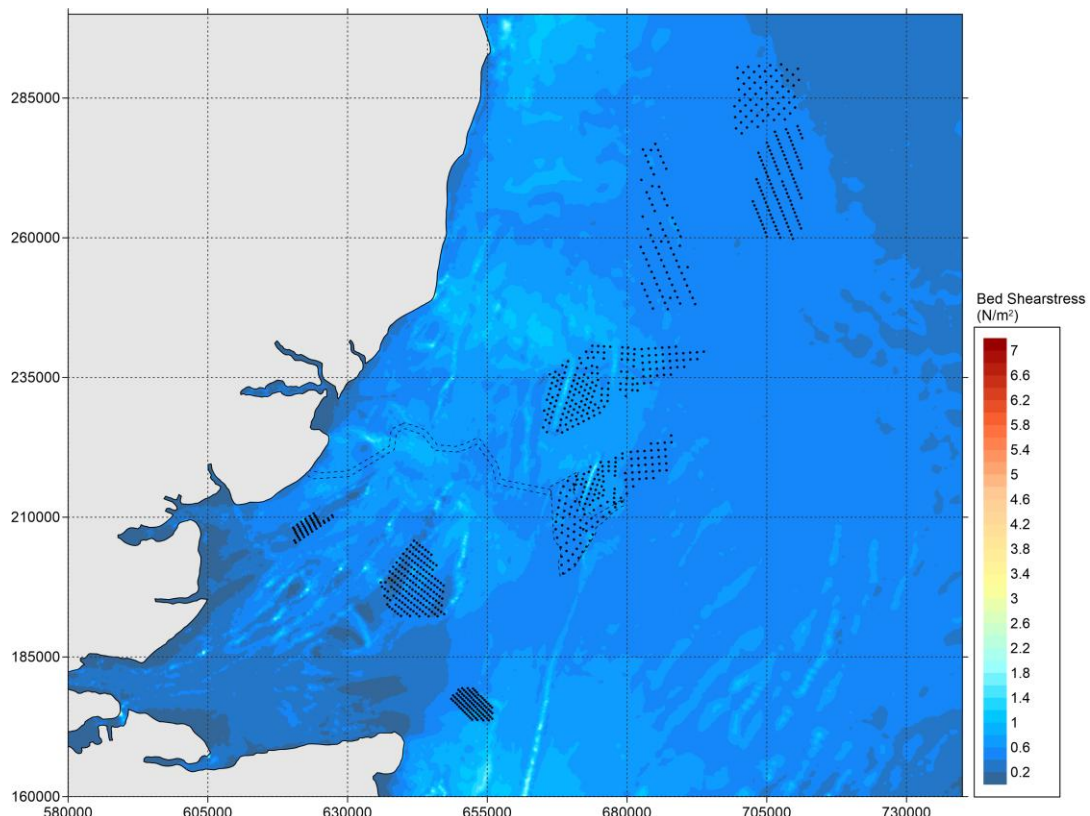
Figure 5.51 All windfarms ('Cumulative') – Bed shear stress during neap tide – peak flood.
