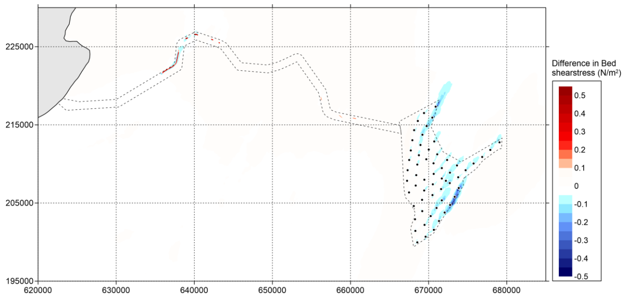
Figure 5.66 Difference in bed shear stress (in \text{N/m}^2 ) between 'Baseline' and 'Option' during spring tide (positive means increase of bed shear stress by option and vice versa) – peak ebb
