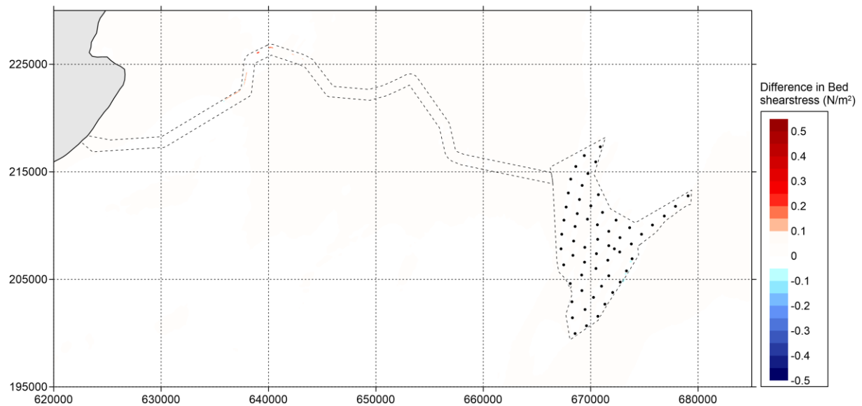
Figure 5.70 Difference in bed shear stress (in \text{N/m}^2 ) between 'Baseline' and 'Option' during neap tide (positive means increase of bed shear stress by option and vice versa) – peak ebb
