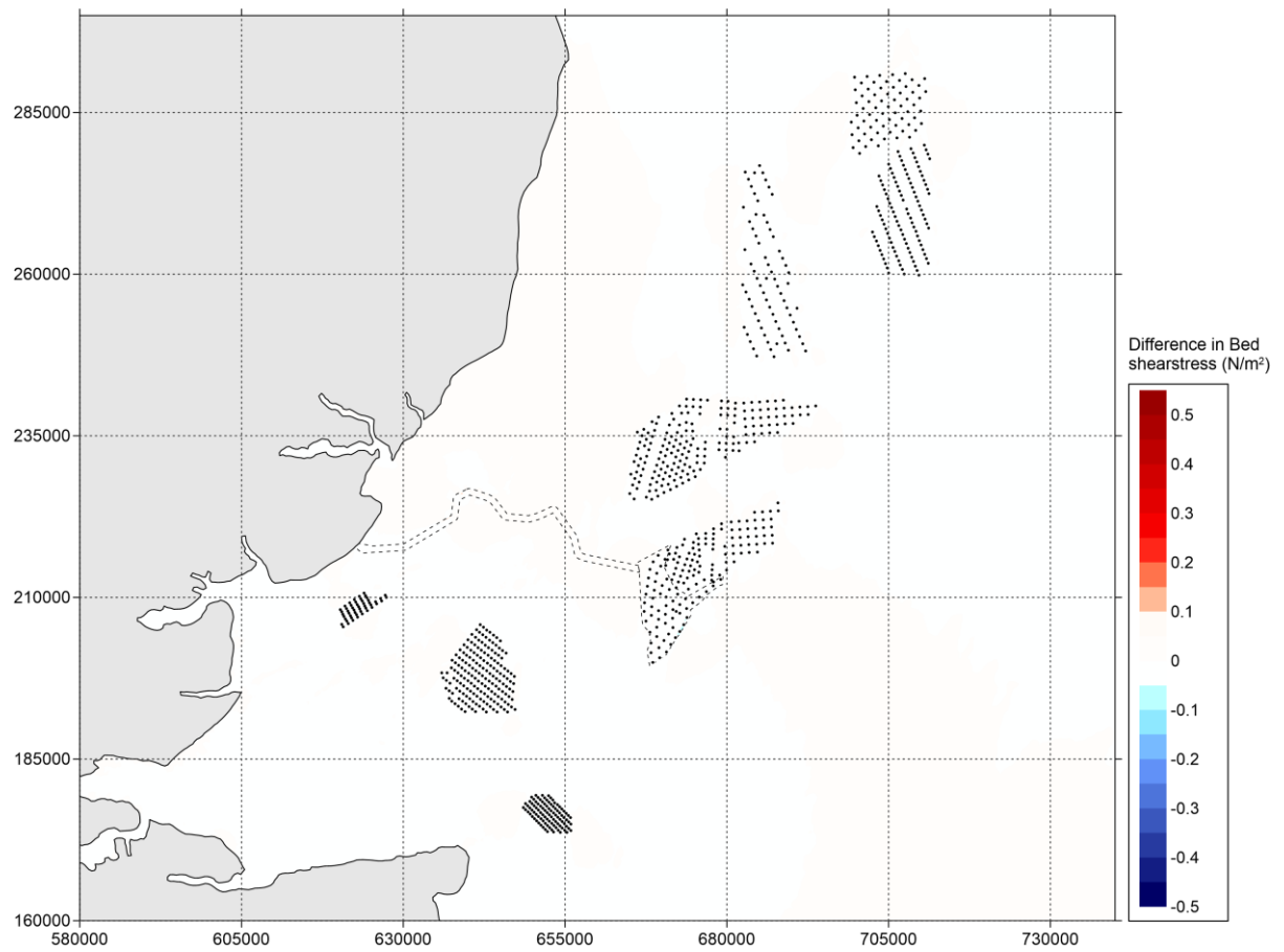
Figure 5.85 Difference in bed shear stress (in \text{N/m}^2 ) between 'Baseline' and 'Cumulative' during neap tide (positive means increase of bed shear stress by option and vice versa) – peak flood.
