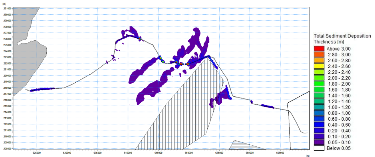
Figure 7.133 Total sediment deposition thickness during export cable levelling operations (including additional length) (vertical hashed area = MLS SAC, horizontal hashed area = KKE MCZ)
