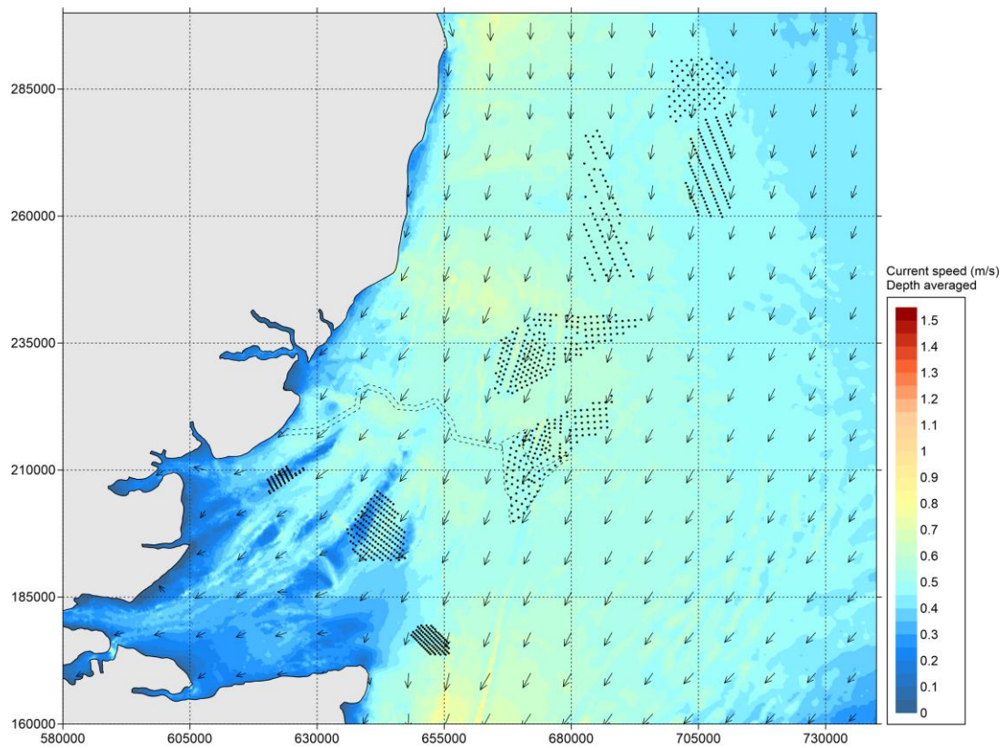
Figure 5.35 All windfarms ('Cumulative') - Current speed during neap tide - peak flood.
