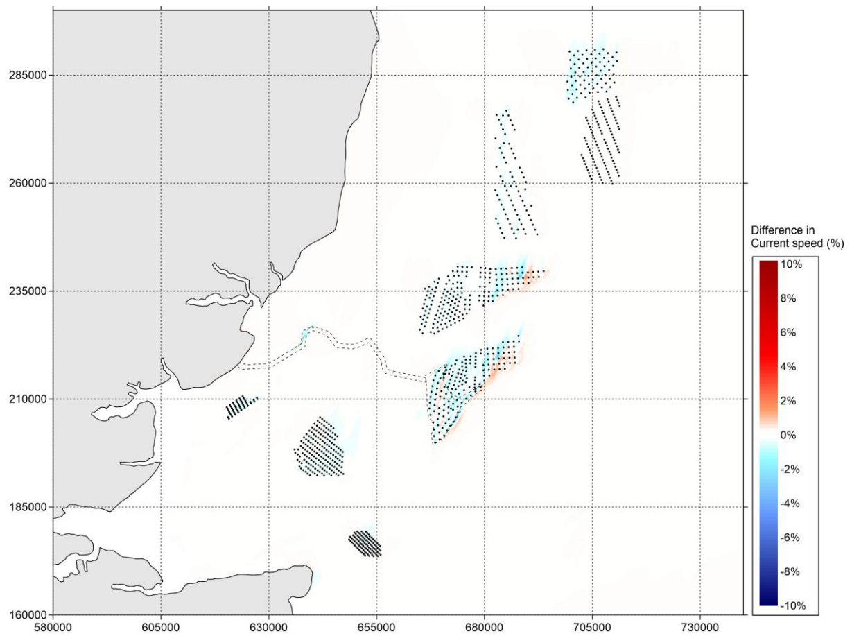
Figure 5.80 Difference in current speed (in percent) between 'Baseline' and 'Cumulative' during neap tide (positive means increase of current speed by option and vice versa) – peak ebb
