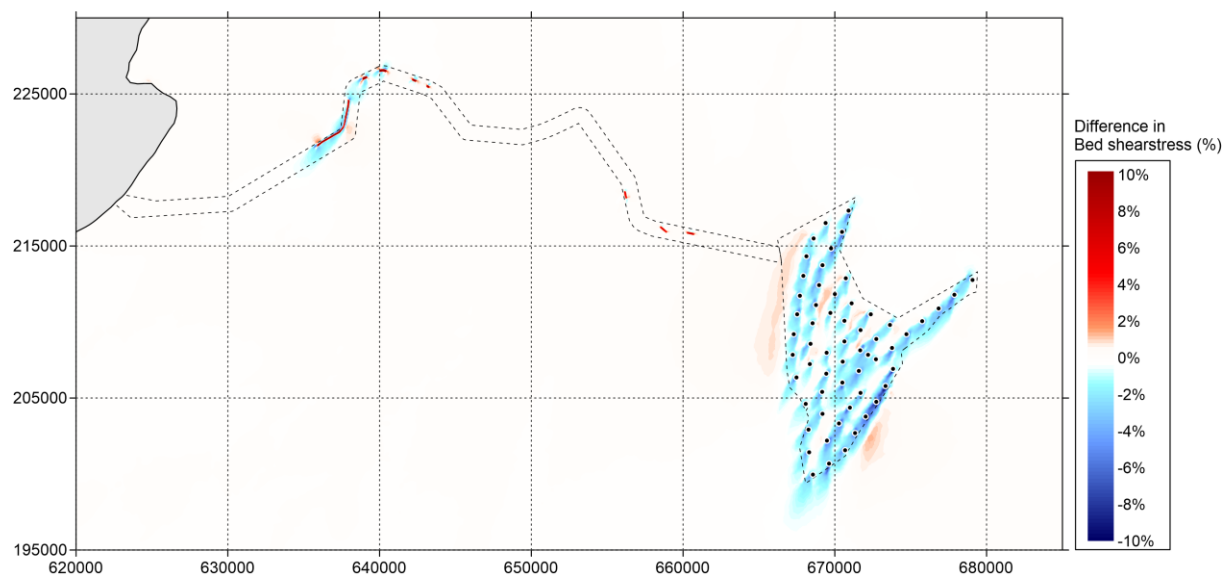
Figure 5.71 Difference in bed shear stress (in percent) between 'Baseline' and 'Option' during neap tide (positive means increase of bed shear stress by option and vice versa) – peak flood
