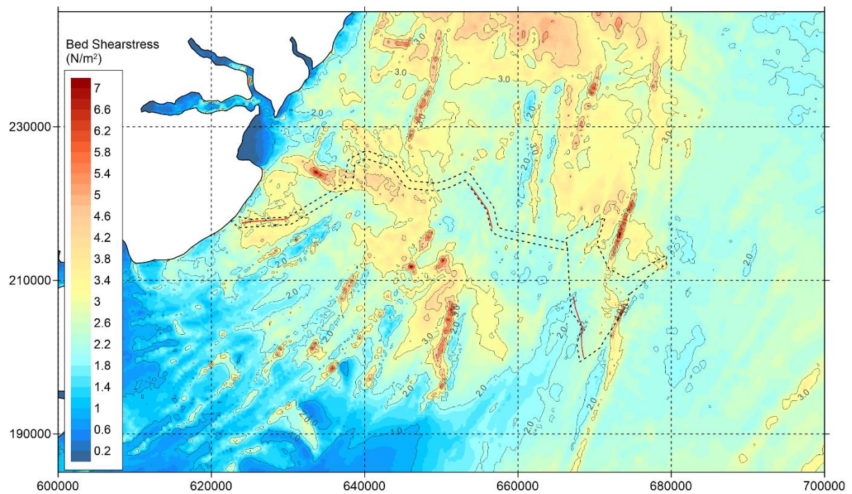
Figure 5.54 'Additional' layout - Bed shear stress during spring tide - peak ebb (zoomed in).
