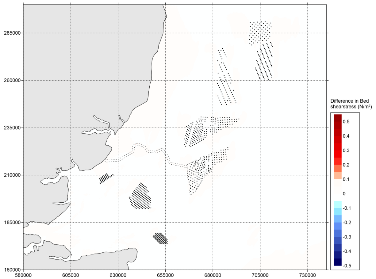
Figure 5.86 Difference in bed shear stress (in \text{N/m}^2 ) between 'Baseline' and 'Cumulative' during neap tide (positive means increase of bed shear stress by option and vice versa) – peak ebb.
