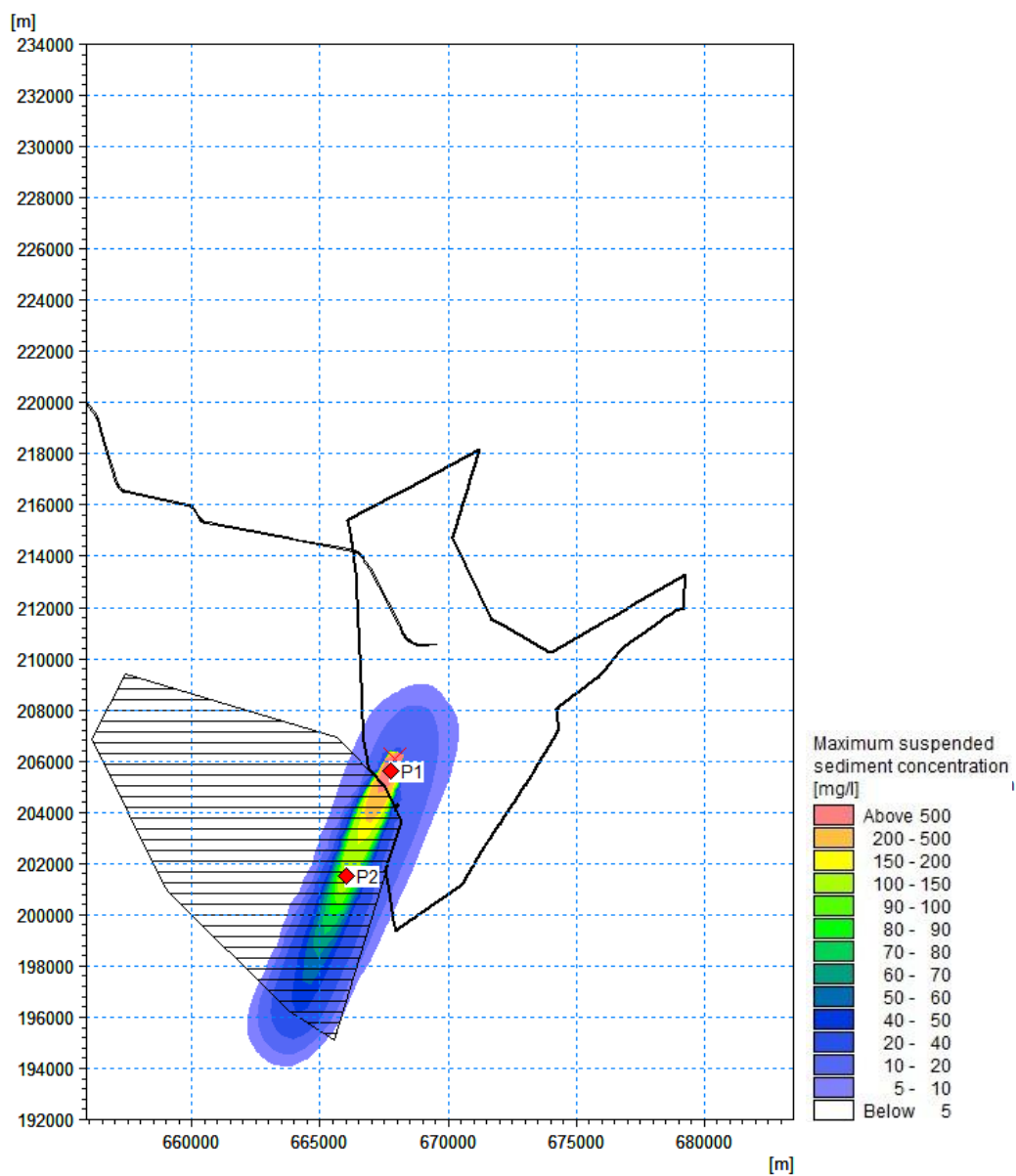
Figure 7.111 Maximum suspended sediment concentration during array disposal occurring near middle of water column– Slack water near low water during neap tide ('Zone 1 & 3' material) (red point = time series extraction point)
