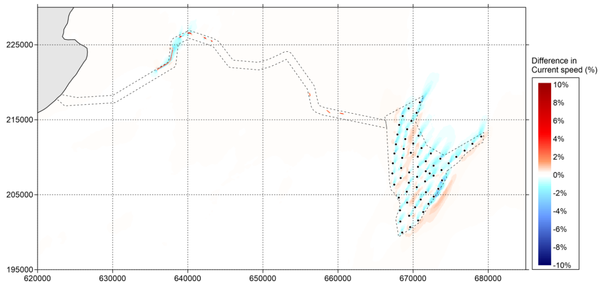
Figure 5.64 Difference in current speed (in percent) between 'Baseline' and 'Option' during neap tide (positive means increase of current speed by option and vice versa) – peak ebb
