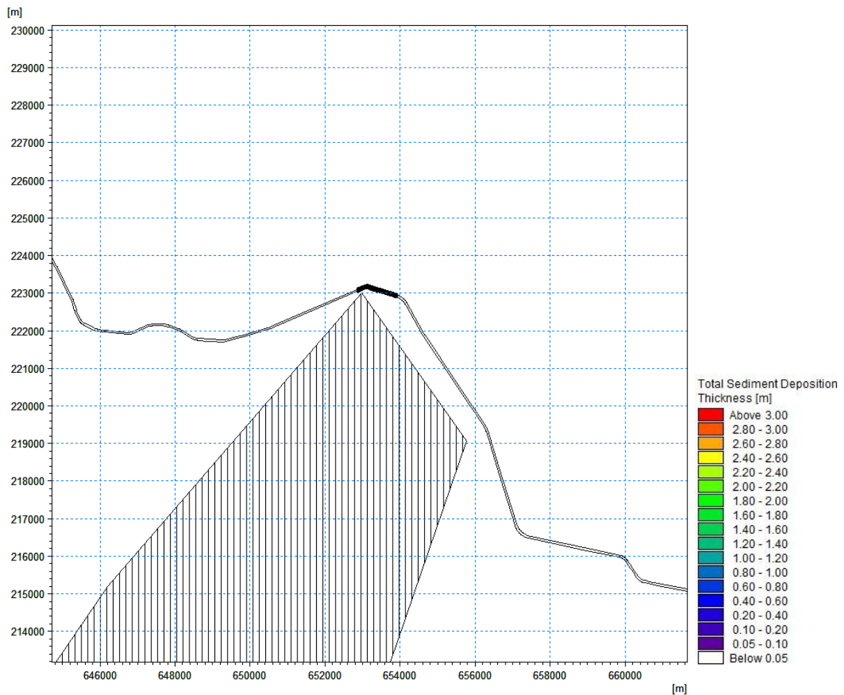
Figure 7.104 Total sediment deposition thickness during dredging operations at Pilot Boarding Area (vertical hashed area = MLS SAC)
