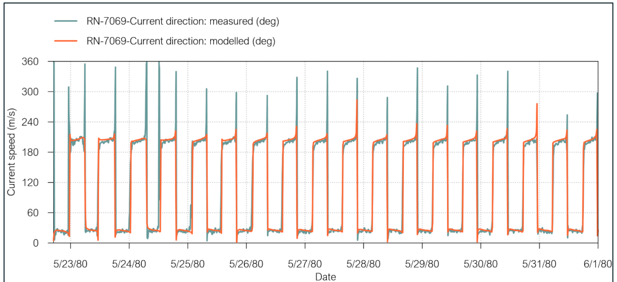
Figure 5.13: Time series comparison between simulated vs observed current directions at RN-7069 station in May 1980 (Local model)
