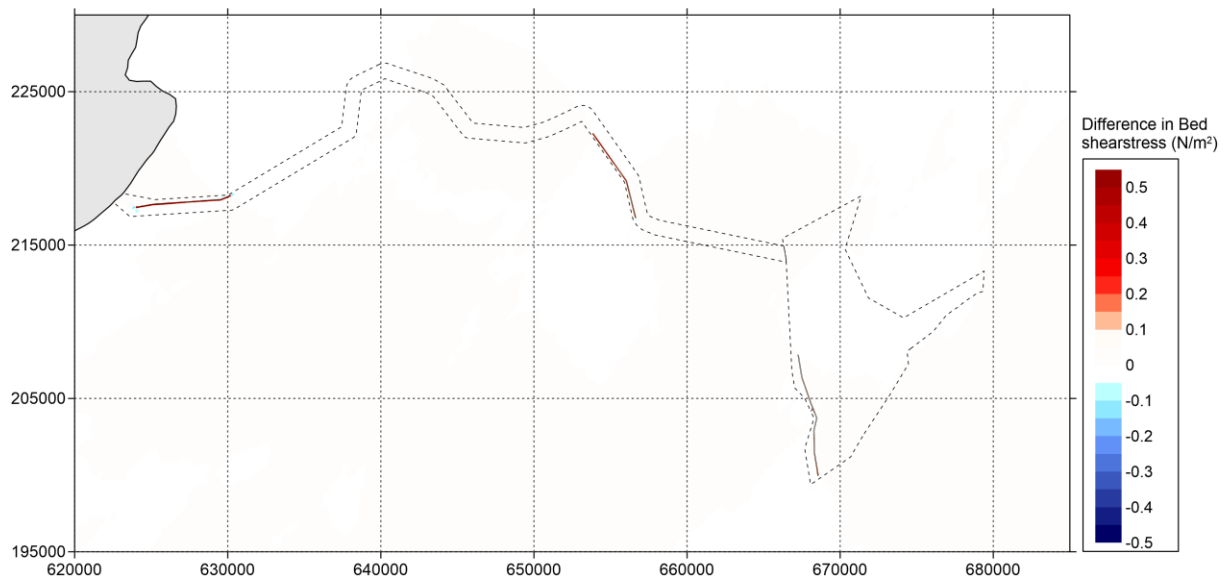
Figure 5.97 Difference in bed shear stress (in \text{N/m}^2 ) between 'Baseline' and 'Additional Layout' during spring tide (positive means increase of bed shear stress by option and vice versa) – peak flood
