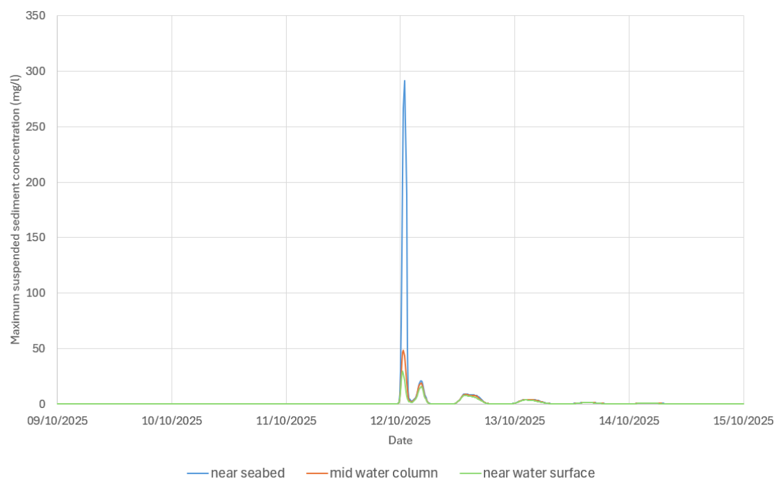
Figure 7.138 Time series of suspended sediment concentration at P2 during indicative offshore export cable levelling (including additional length), array cable levelling and seabed preparation operations for smaller WTGs layout structures for seabed, middle of water column and near water surface (inside KKE MCZ)
