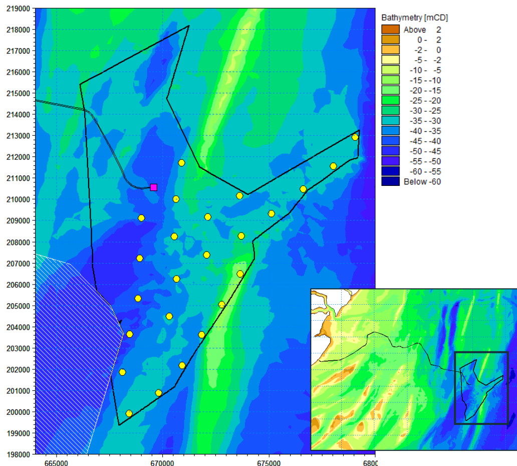
Figure 6.9 Location of seabed preparation activities for array structures – larger WTGs indicative Layout (purple square = OCP/OSP, yellow dot = WTGs, white hatch = MCZ)
