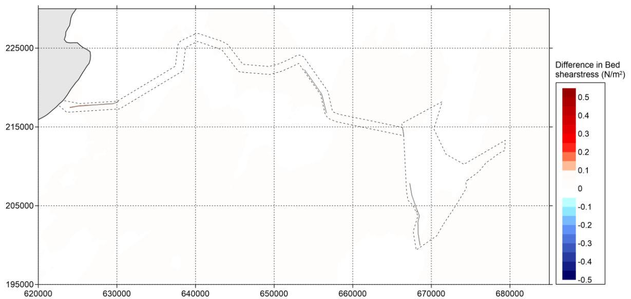
Figure 5.102 Difference in bed shear stress (in \text{N/m}^2 ) between 'Baseline' and 'Additional Layout' during neap tide (positive means increase of bed shear stress by option and vice versa) – peak ebb.
