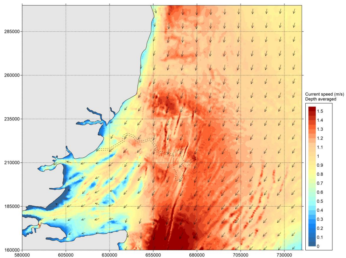
Figure 5.22 Baseline - Current speed during spring tide - peak flood (zoomed out)
