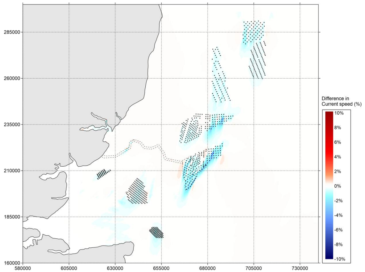
Figure 5.75 Difference in current speed (in percent) between 'Baseline' and 'Cumulative' during spring tide (positive means increase of current speed by option and vice versa) – peak flood
