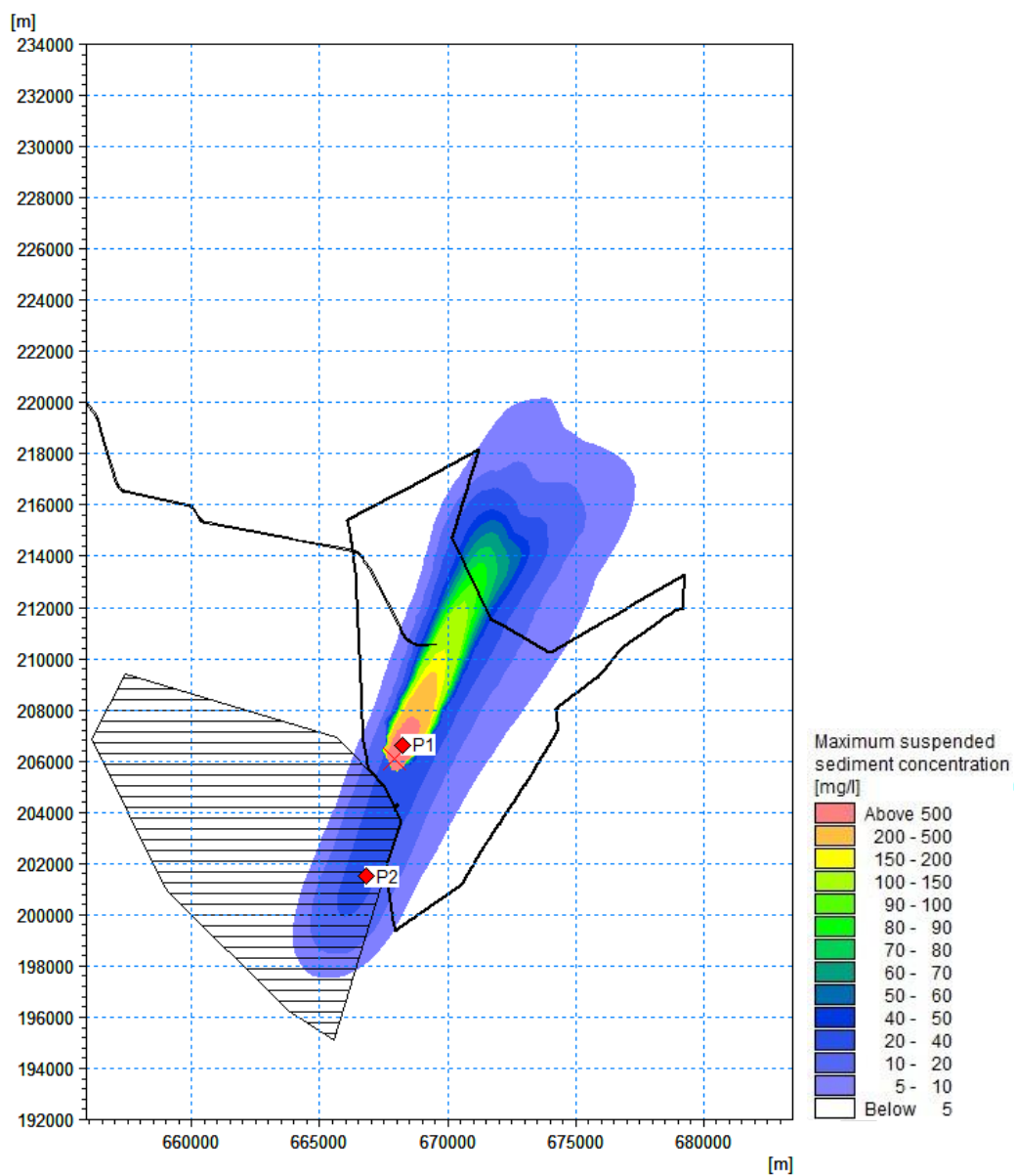
Figure 7.124 Maximum suspended sediment concentration during array disposal occurring near the water surface – Peak ebb during spring tide ('Zone 1 & 3' material) (red point = time series extraction point)
