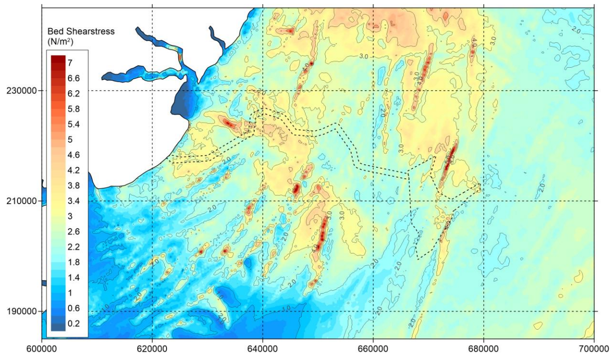
Figure 5.39 Baseline – Bed shear stress during spring tide - peak ebb (zoomed in).
