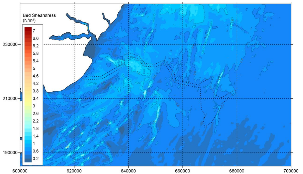
Figure 5.43 Baseline – Bed shear stress during neap tide - peak ebb (zoomed in).
