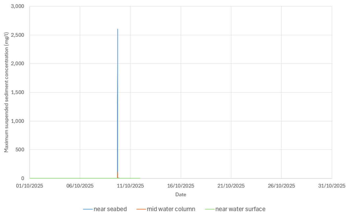
Figure 7.34 Time series of suspended sediment concentration at P1 during seabed preparation for array structures (smaller WTGs) near seabed, middle of water column and near water surface (near MCZ)
