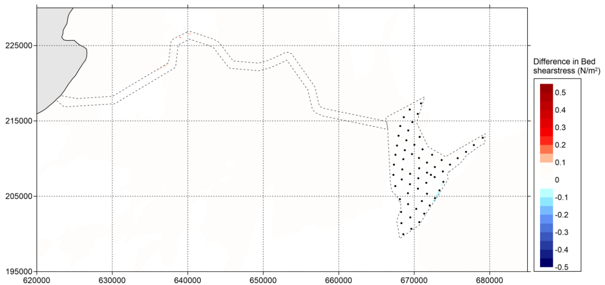
Figure 5.69 Difference in bed shear stress (in \text{N/m}^2 ) between 'Baseline' and 'Option' during neap tide (positive means increase of bed shear stress by option and vice versa) – peak flood
