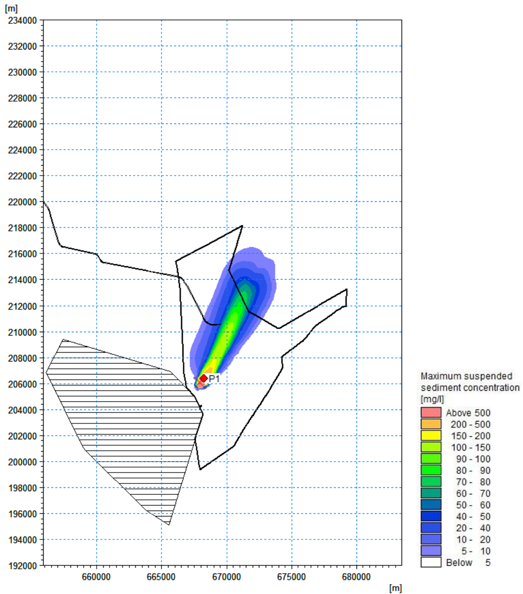
Figure 7.105 Maximum suspended sediment concentration during array disposal occurring near the seabed – Slack water near high water during neap tide ('Zone 1 & 3' material) (red point = time series extraction point)
