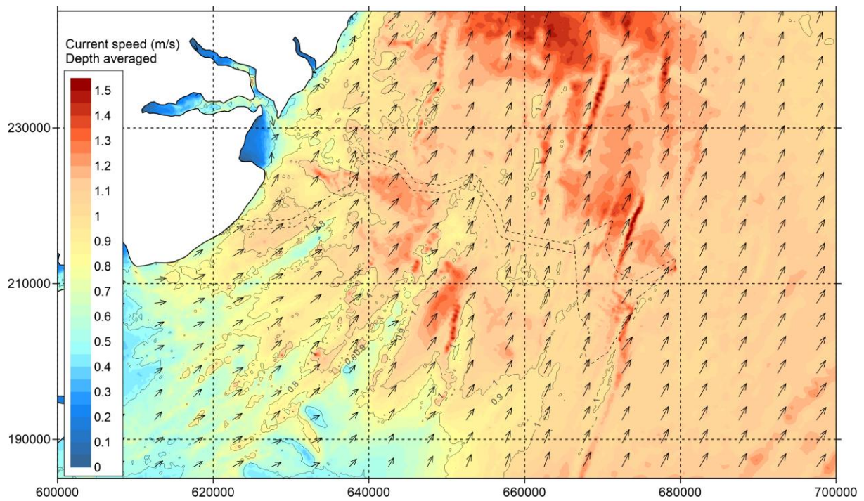
Figure 5.23 Baseline - Current speed during spring tide - peak ebb (zoomed in).
