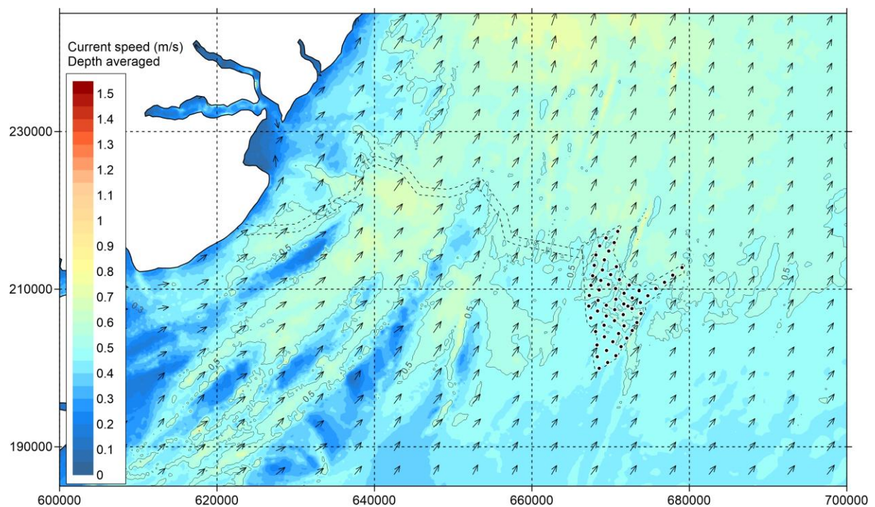
Figure 5.32 Option - Current speed during neap tide - peak ebb.
