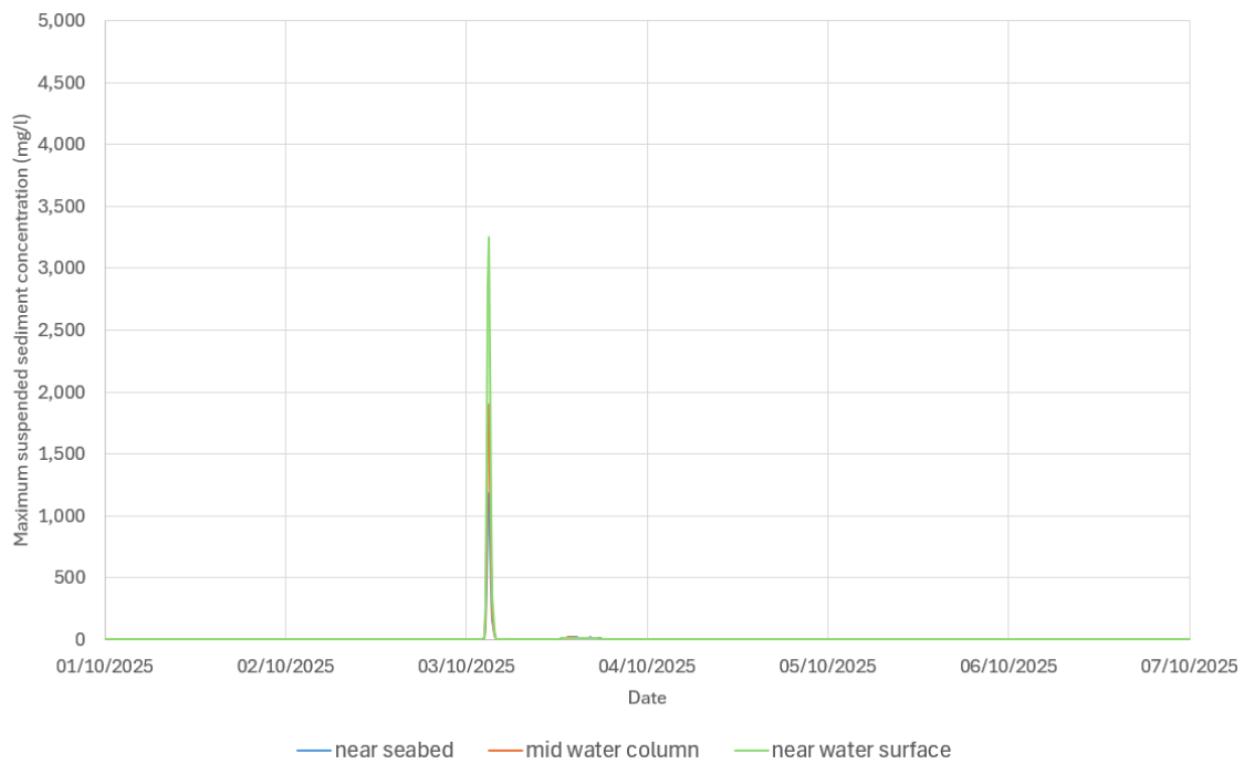
Figure 7.113 Time series of suspended sediment concentration at P1 during sediment disposal near seabed, middle of water column and near water surface - Slack water near low water during neap tide ('Zone 1 & 3' material)
