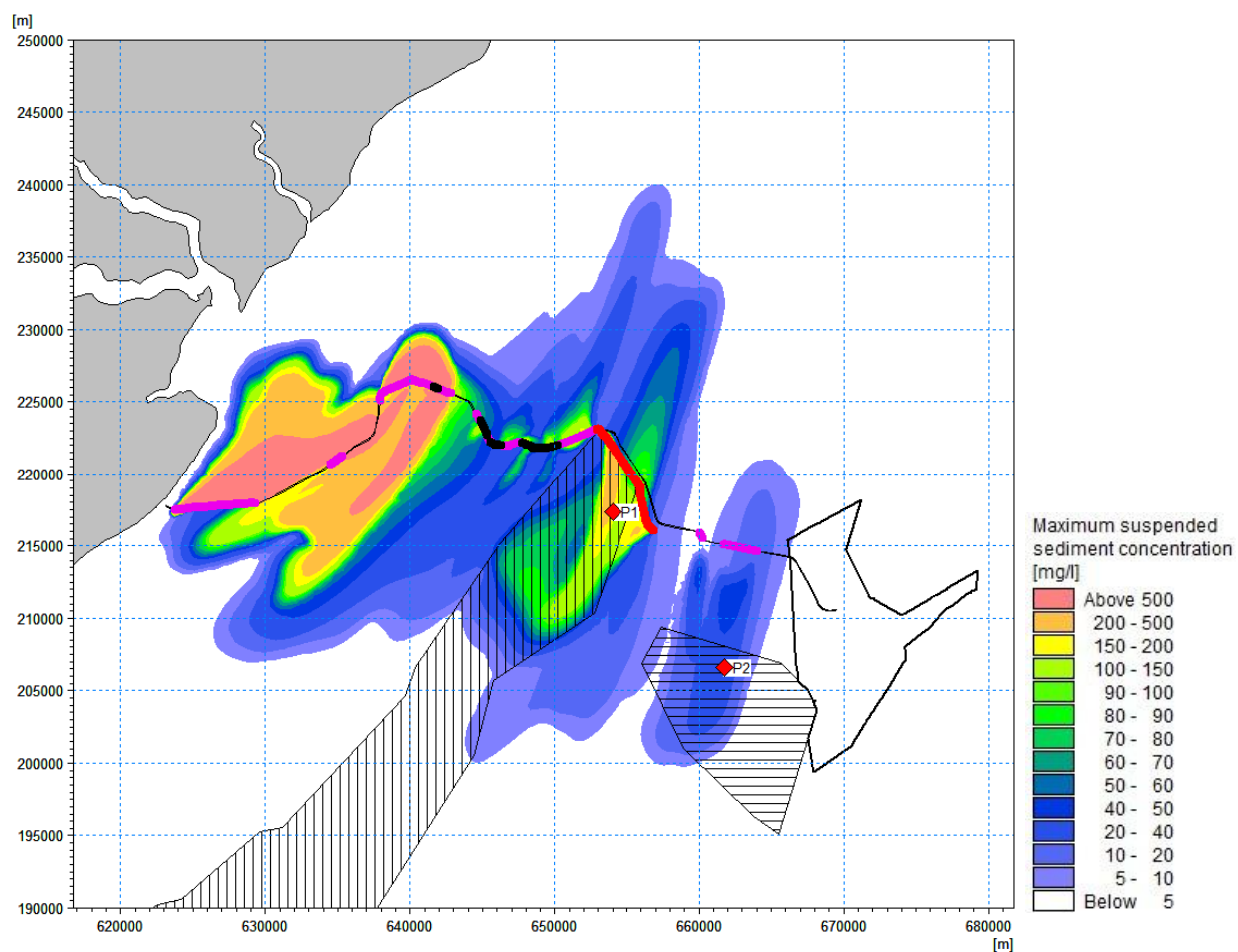
Figure 7.130 Maximum suspended sediment concentration during an indicative offshore export cable levelling (including additional length) near the water surface (thick purple line = MR, thick black line = SW, red points = time series extraction points, vertical hashed area = MLS SAC, horizontal hashed area = KKE MCZ)
