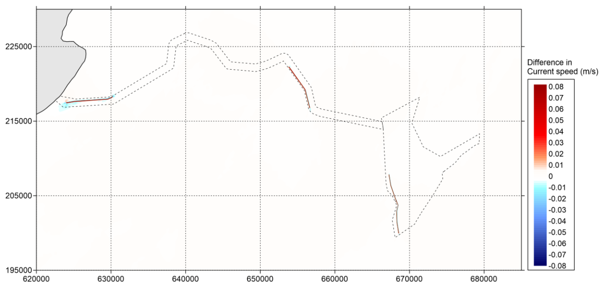
Figure 5.89 Difference in current speed (in metres/second) between 'Baseline' and 'Additional Layout' during spring tide (positive means increase of current speed by option and vice versa) – peak flood
