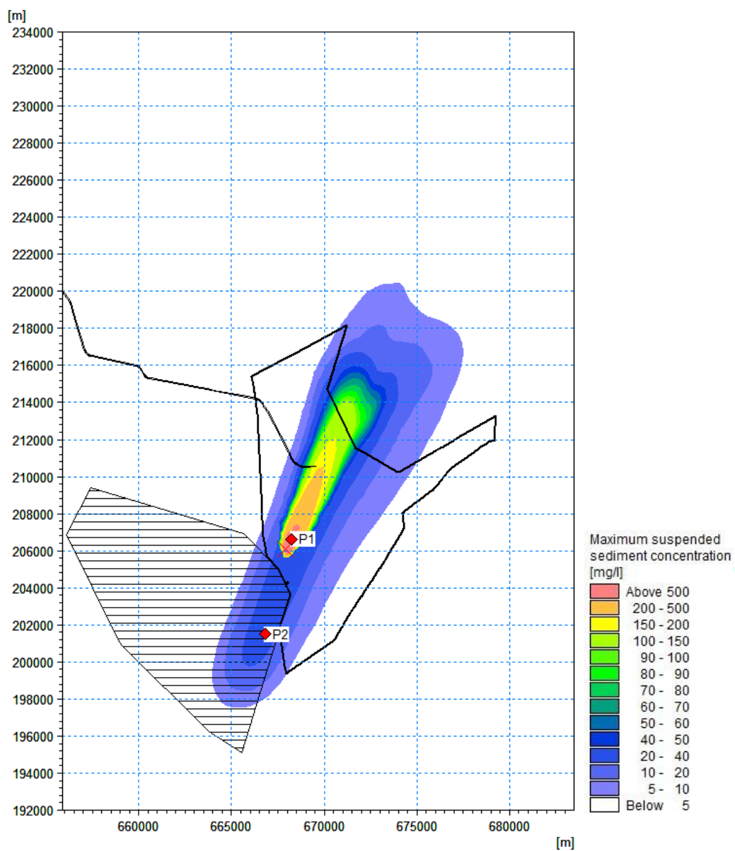
Figure 7.123 Maximum suspended sediment concentration during array disposal occurring near the middle of water column – Peak ebb during spring tide ('Zone 1 & 3' material) (red point = time series extraction point)
