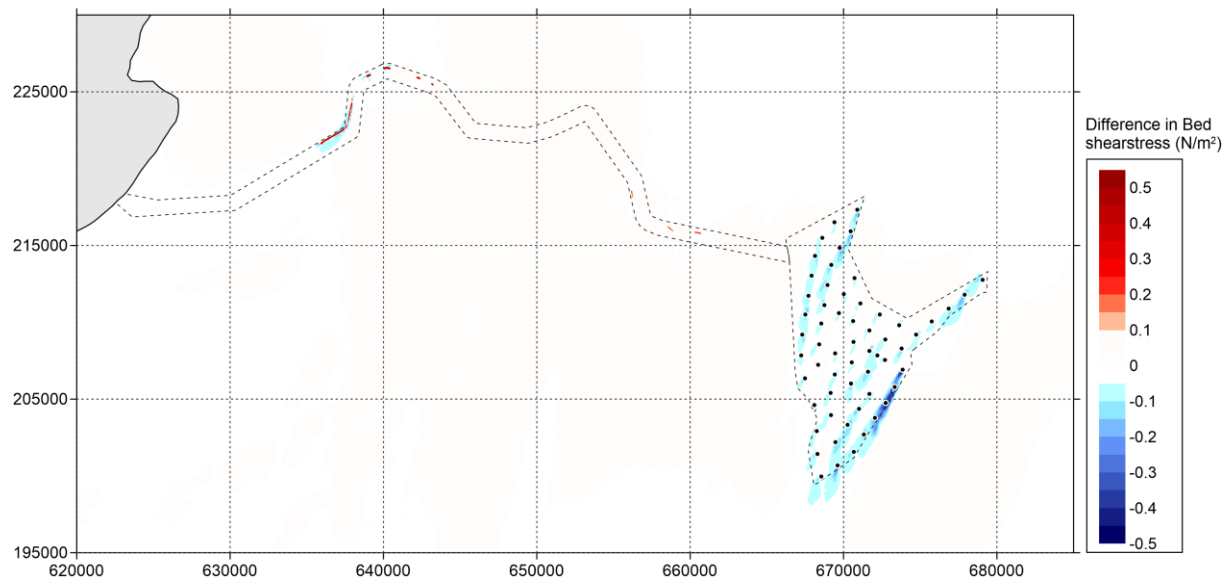
Figure 5.65 Difference in bed shear stress (in \text{N/m}^2 ) between 'Baseline' and 'Option' during spring tide (positive means increase of bed shear stress by option and vice versa) – peak flood
