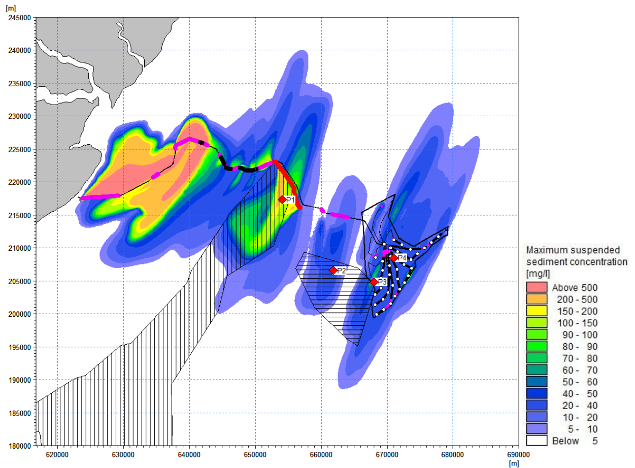
Figure 7.136 Maximum suspended sediment concentration during an indicative offshore export cable levelling (including additional length), array cable levelling and seabed preparation operations for smaller WTGs layout structures occurring near the water surface (thick purple line = MR, thick black line = SW, white points = WTG structures, red points = time series extraction points, vertical hashed area = MLS SAC, horizontal hashed area = KKE MCZ)
