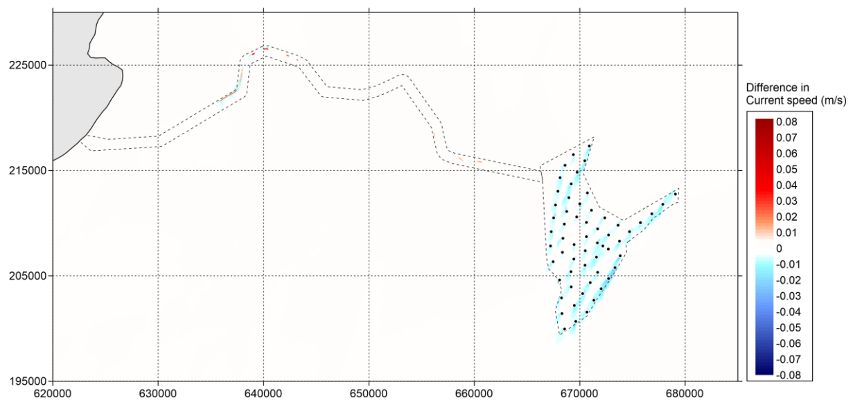
Figure 5.61 Difference in current speed (in metres/second) between 'Baseline' and 'Option' during neap tide (positive means increase of current speed by option and vice versa) – peak flood
