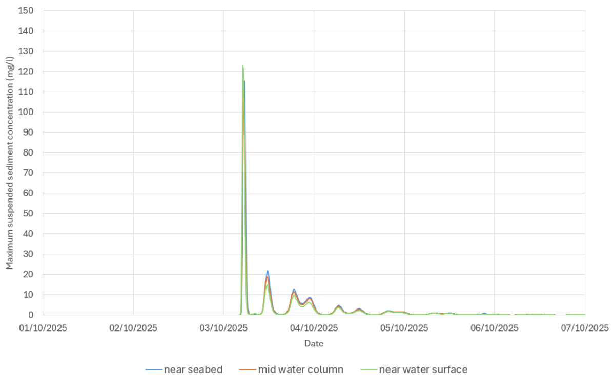
Figure 7.114 Time series of suspended sediment concentration at P2 during sediment disposal near seabed, middle of water column and near water surface - Slack water near low water during neap tide ('Zone 1 & 3' material)
