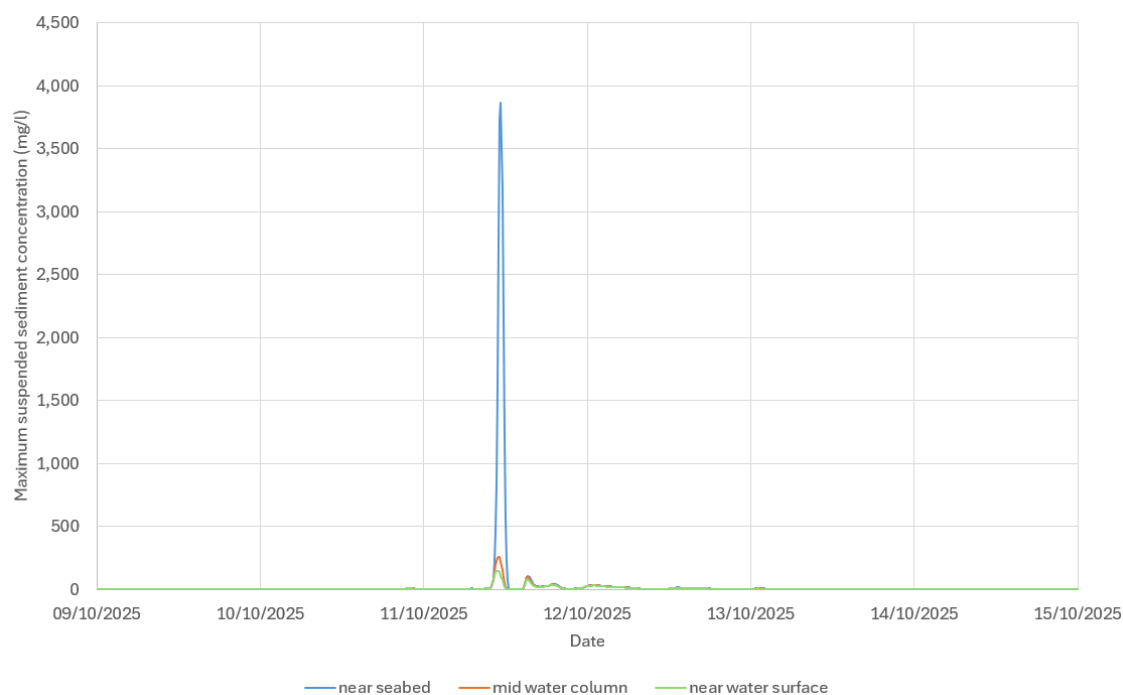
Figure 7.137 Time series of suspended sediment concentration at P1 during indicative offshore export cable levelling (including additional length), array cable levelling and seabed preparation operations for smaller WTGs layout structures for seabed, middle of water column and near water surface (inside MLS SAC)
