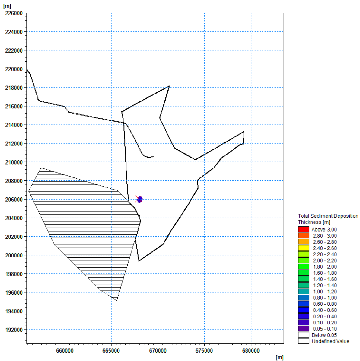
Figure 7.109 Total deposition thickness during sediment disposal - Slack water near high water during neap tide ('Zone 1 & 3' material)
