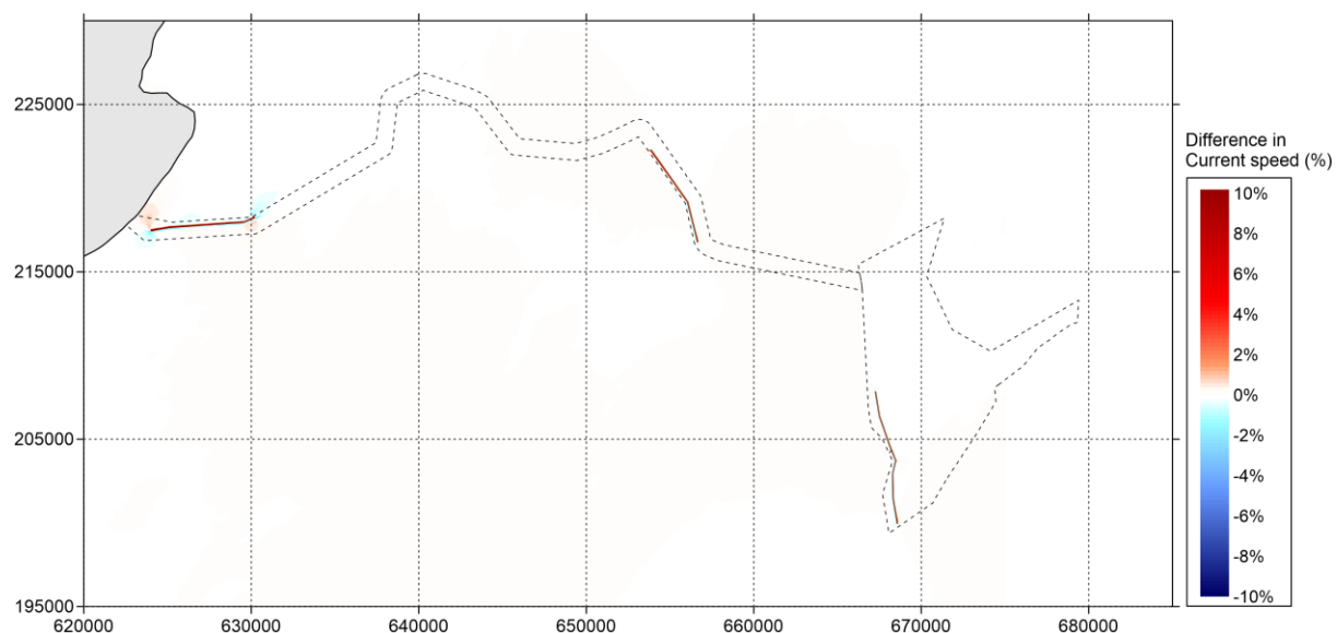
Figure 5.92 Difference in current speed (in percent) between 'Baseline' and 'Additional Layout' during spring tide (positive means increase of current speed by option and vice versa) – peak ebb
