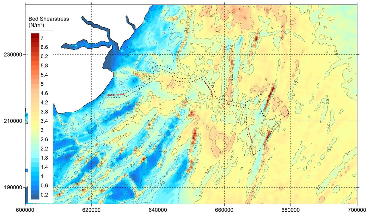
Figure 5.53 'Additional' layout – Bed shear stress during spring tide - peak flood (zoomed in).
