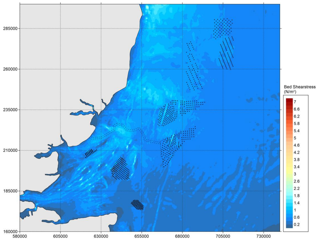
Figure 5.52 All windfarms ('Cumulative') – Bed shear stress during neap tide – peak ebb.
