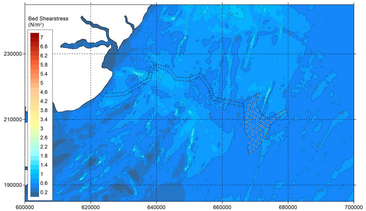
Figure 5.47 Option – Bed shear stress during neap tide - peak flood.
