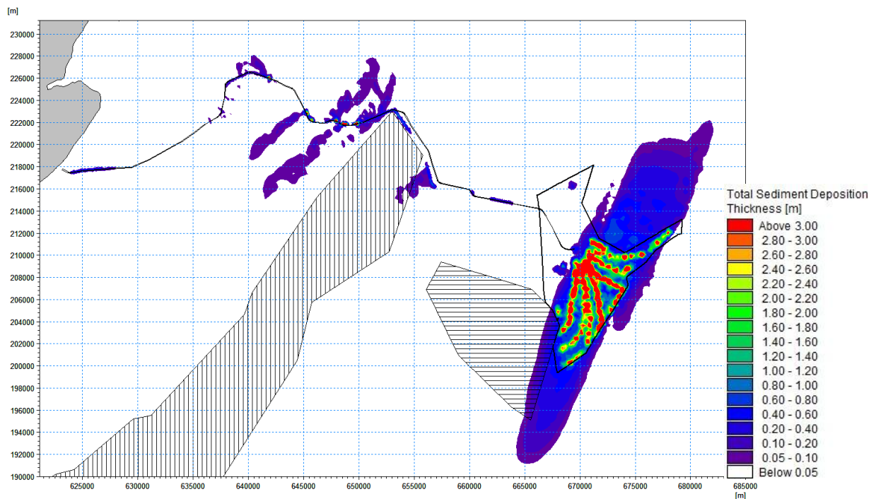
Figure 7.141 Total sediment deposition thickness during an indicative offshore export cable levelling (including additional length), array cable levelling and seabed preparation operations for smaller WTGs layout structures (vertical hashed area = MLS SAC, horizontal hashed area = KKE MCZ)
