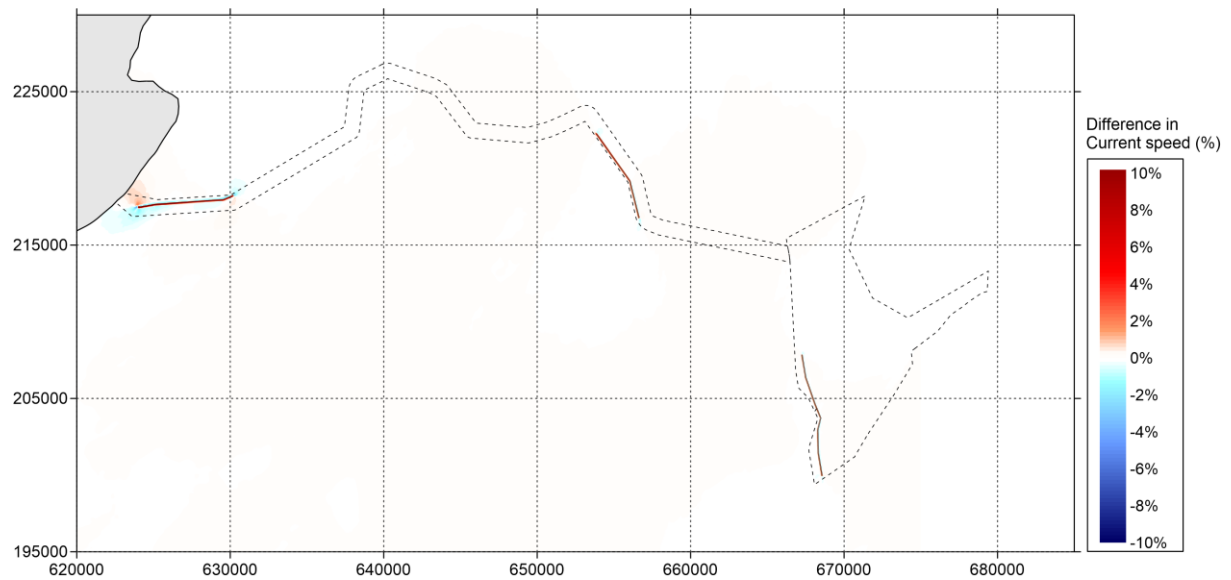
Figure 5.95 Difference in current speed (in percent) between 'Baseline' and 'Additional Layout' during neap tide (positive means increase of current speed by option and vice versa) – peak flood
