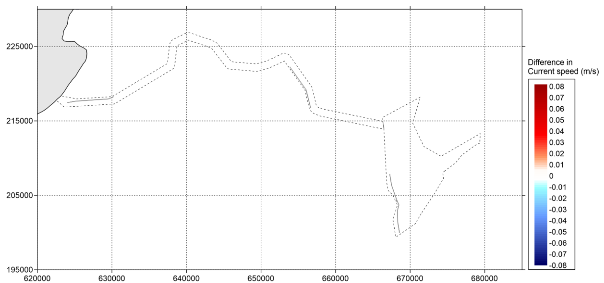
Figure 5.94 Difference in current speed (in metres/second) between 'Baseline' and 'Additional Layout' during neap tide (positive means increase of current speed by option and vice versa) – peak ebb
