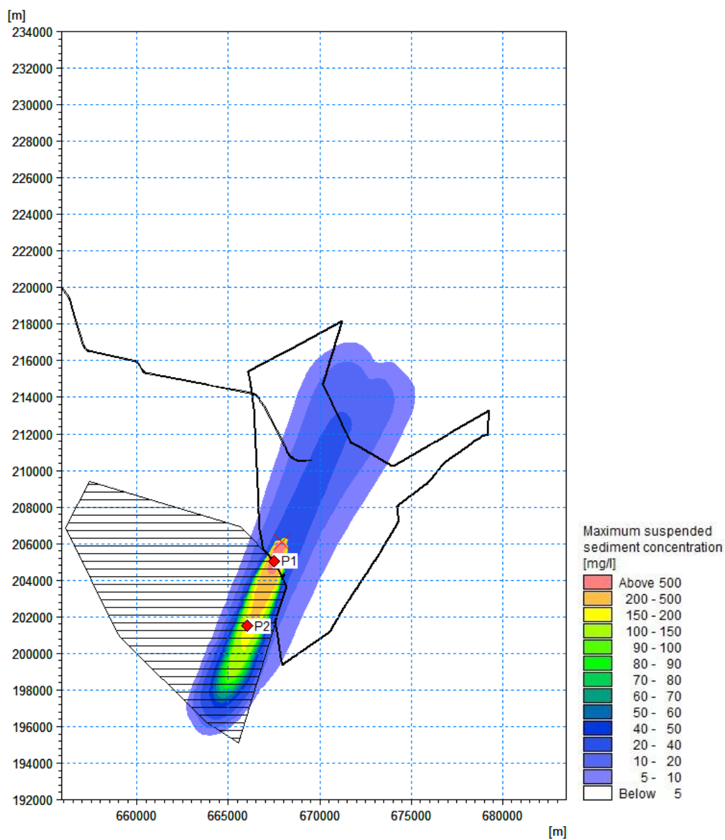
Figure 7.117 Maximum suspended sediment concentration during array disposal occurring near the middle of water column – Peak flood during spring tide ('Zone 1 & 3' material) (red point = time series extraction point)
