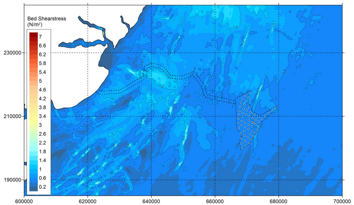
Figure 5.48 Option – Bed shear stress during neap tide - peak ebb.
