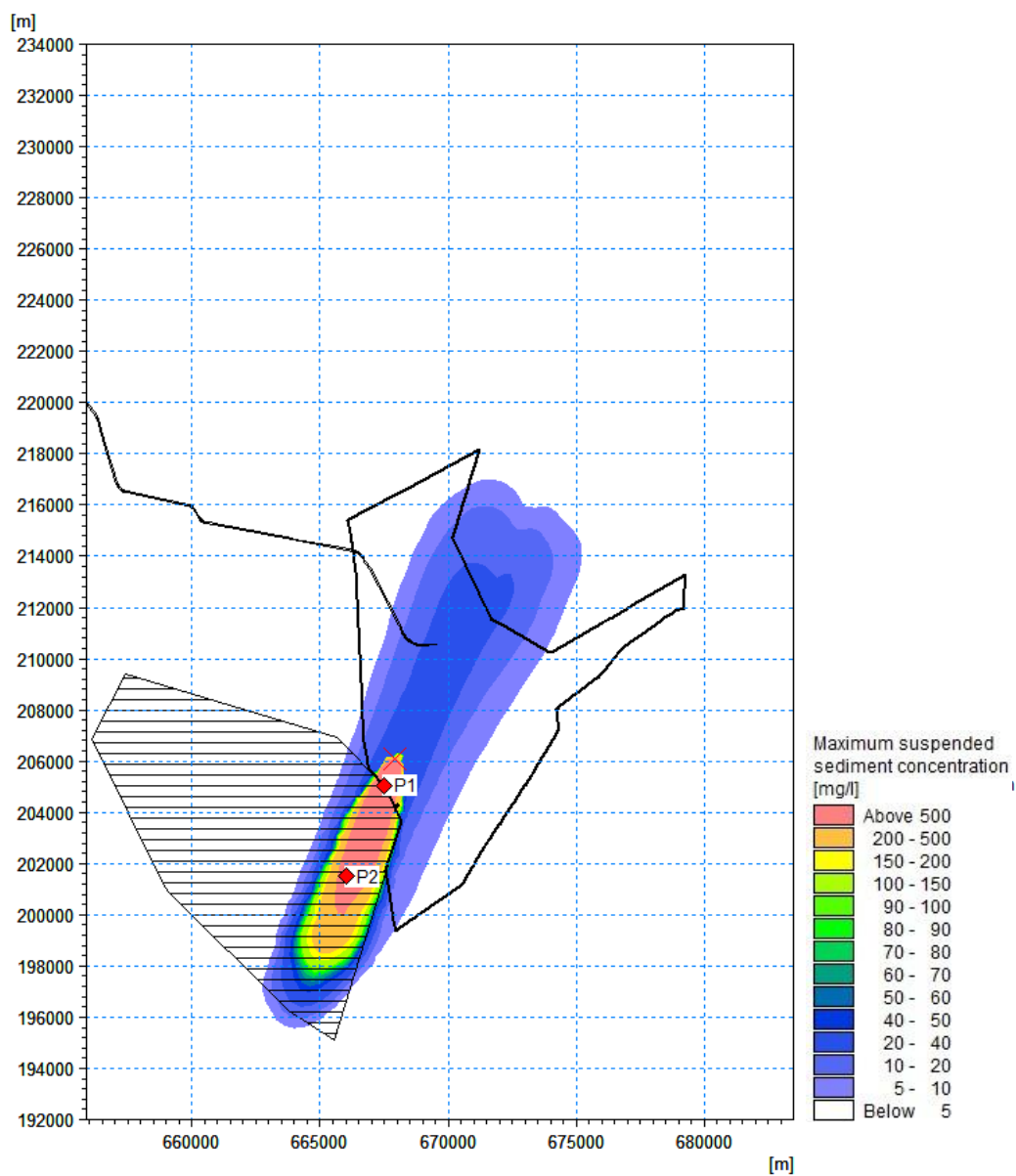
Figure 7.116 Maximum suspended sediment concentration during array disposal occurring near the seabed – Peak flood during spring tide ('Zone 1 & 3' material) (red point = time series extraction point)
