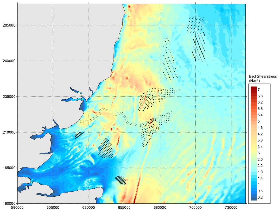
Figure 5.50 All windfarms ('Cumulative') – Bed shear stress during spring tide – peak ebb
