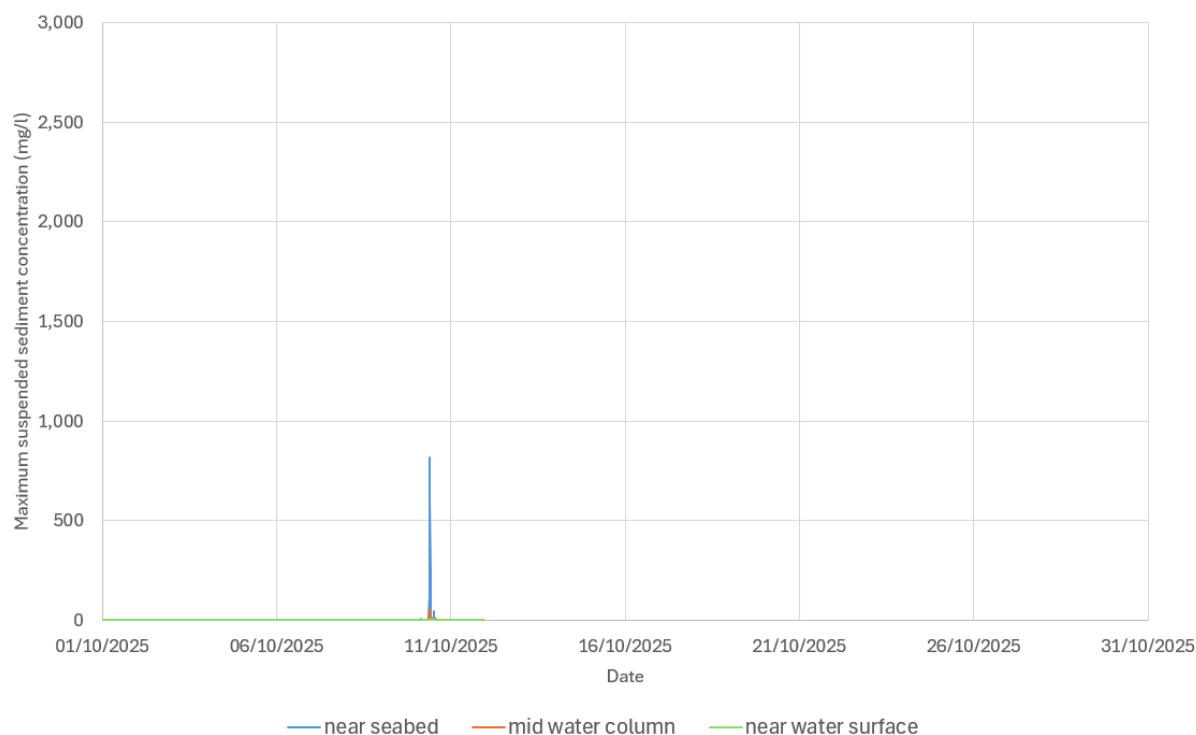
Figure 7.40 Time series of suspended sediment concentration at P1 during seabed preparation for array structures (larger WTGs) near seabed, middle of water column and near water surface
