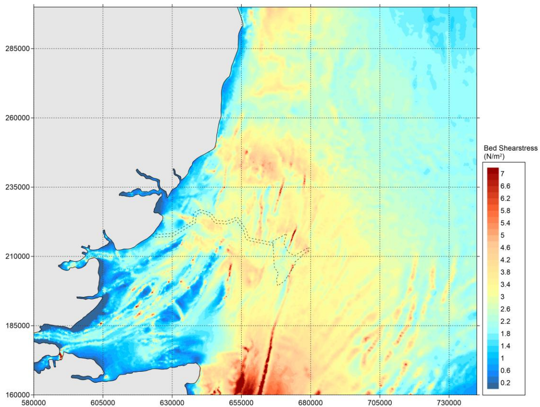
Figure 5.38 Baseline – Bed shear stress during spring tide - peak flood (zoomed out).
