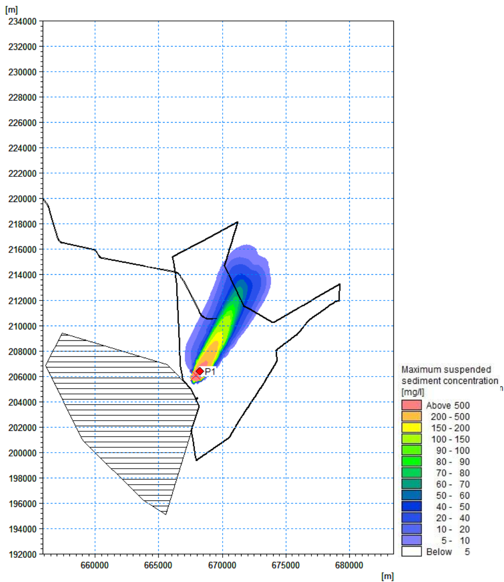
Figure 7.107 Maximum suspended sediment concentration during array disposal occurring near the water surface – Slack water near high water during neap tide ('Zone 1 & 3' material) (red point = time series extraction point)
