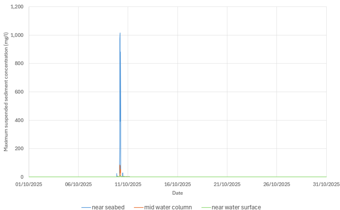
Figure 7.41 Time series of suspended sediment concentration at P2 during seabed preparation for array structures (larger WTGs) near seabed, middle of water column and near water surface
