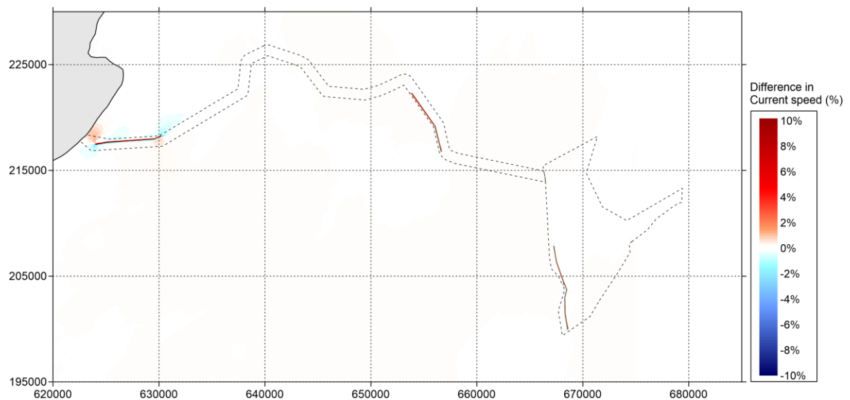
Figure 5.96 Difference in current speed (in percent) between 'Baseline' and 'Additional Layout' during neap tide (positive means increase of current speed by option and vice versa) – peak ebb
