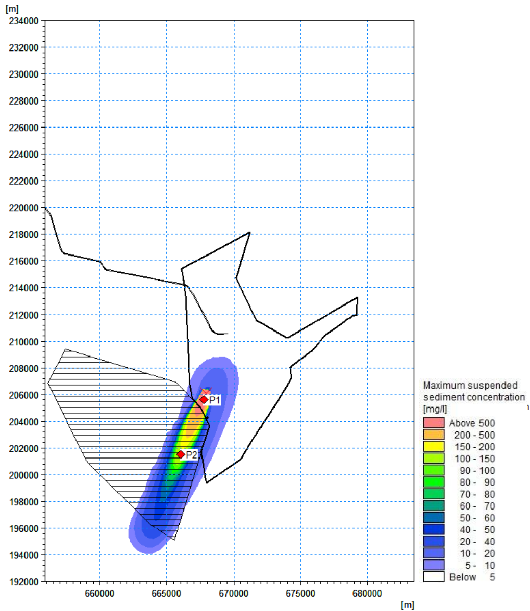
Figure 7.112 Maximum suspended sediment concentration during array disposal occurring near the water surface – Slack water near low water during neap tide ('Zone 1 & 3' material) (red point = time series extraction point)
