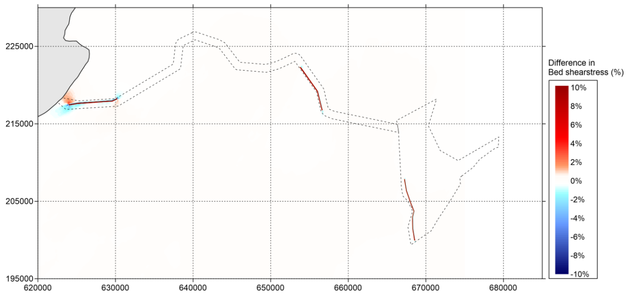
Figure 5.103 Difference in bed shear stress (in percent) between 'Baseline' and 'Additional Layout' during neap tide (positive means increase of bed shear stress by option and vice versa) – peak flood.
