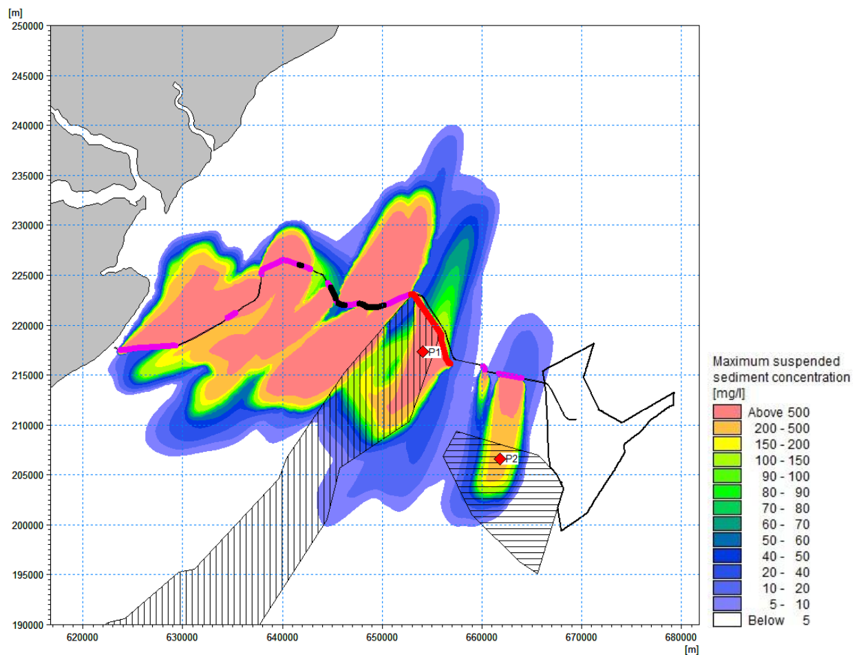
Figure 7.128 Maximum suspended sediment concentration during an indicative offshore export cable levelling (including additional length) near the seabed (thick purple line = MR, thick black line = SW, red points = time series extraction points, vertical hashed area = MLS SAC, horizontal hashed area = KKE MCZ)
