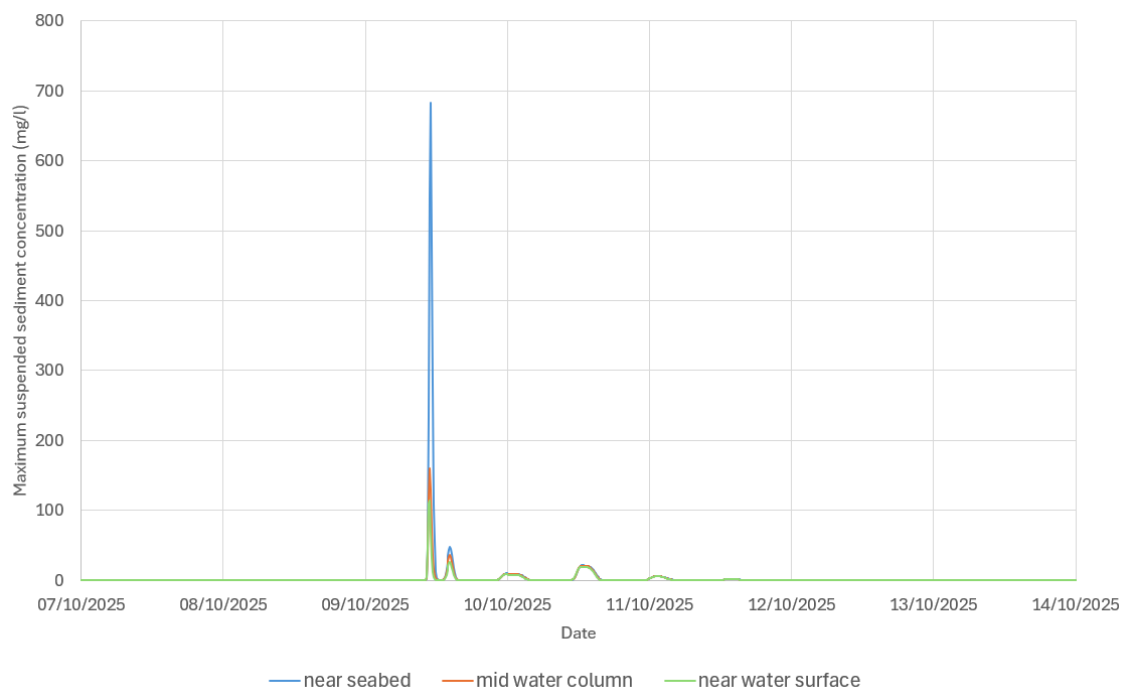
Figure 7.120 Time series of suspended sediment concentration at P2 during sediment disposal near seabed, middle of water column and near water surface – Peak flood during spring tide ('Zone 1 & 3' material)
