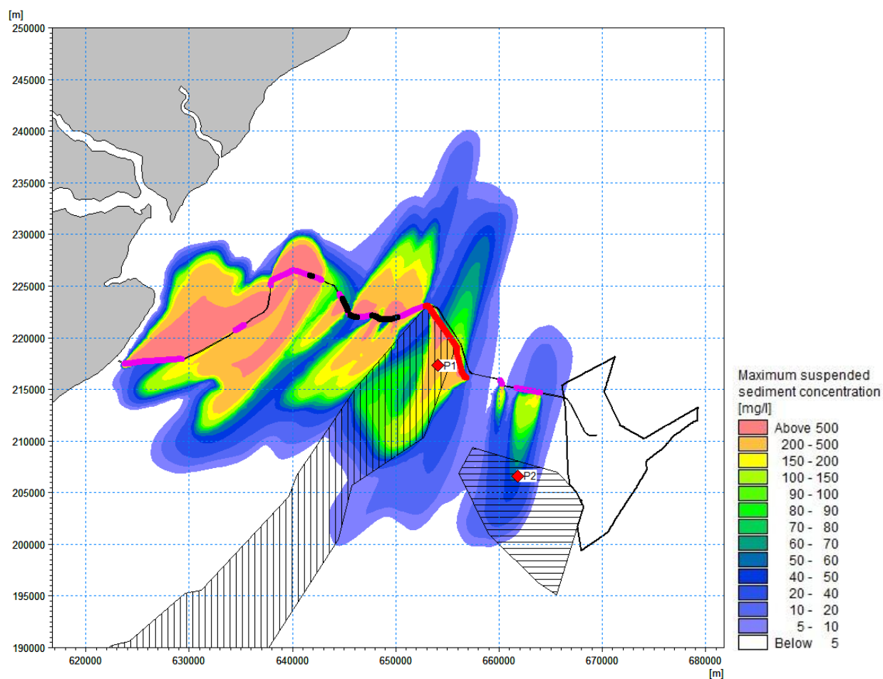
Figure 7.129 Maximum suspended sediment concentration during an indicative offshore export cable levelling (including additional length) in the middle of water column (thick purple line = MR, thick black line = SW, red points = time series extraction points, vertical hashed area = MLS SAC, horizontal hashed area = KKE MCZ)
