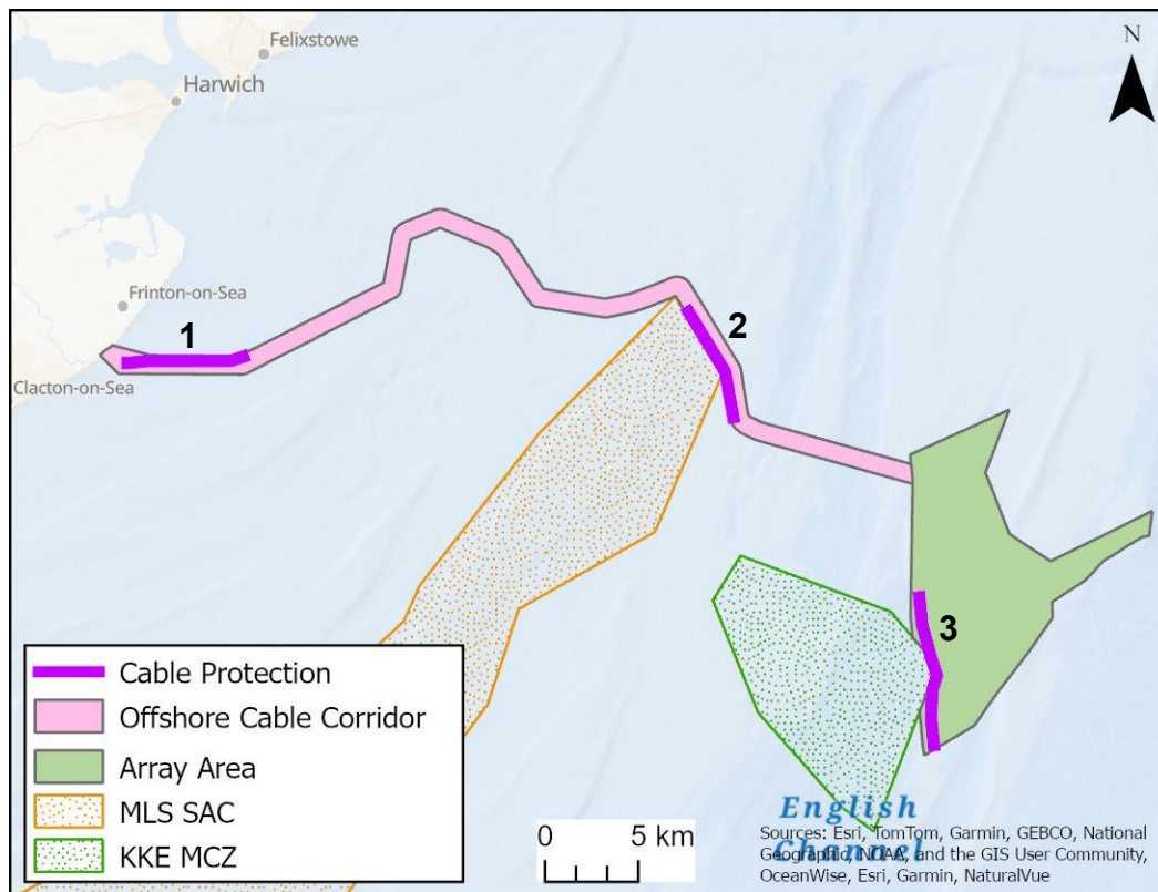
Figure 5.20 Additional layout for three lengths of cable protection
