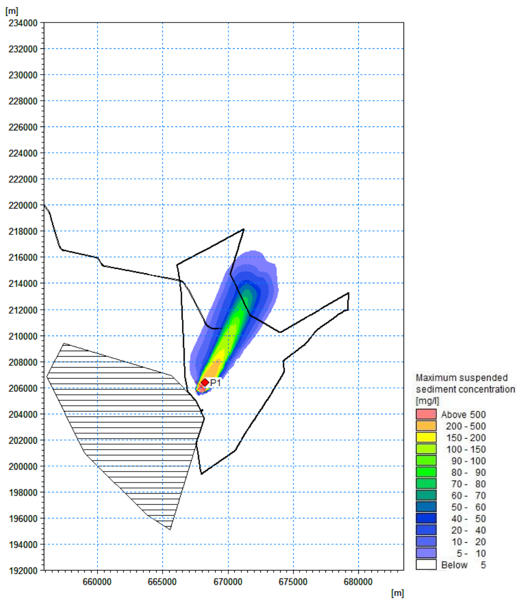
Figure 7.106 Maximum suspended sediment concentration during array disposal occurring near middle of water column– Slack water near high water during neap tide ('Zone 1 & 3' material) (red point = time series extraction point)
