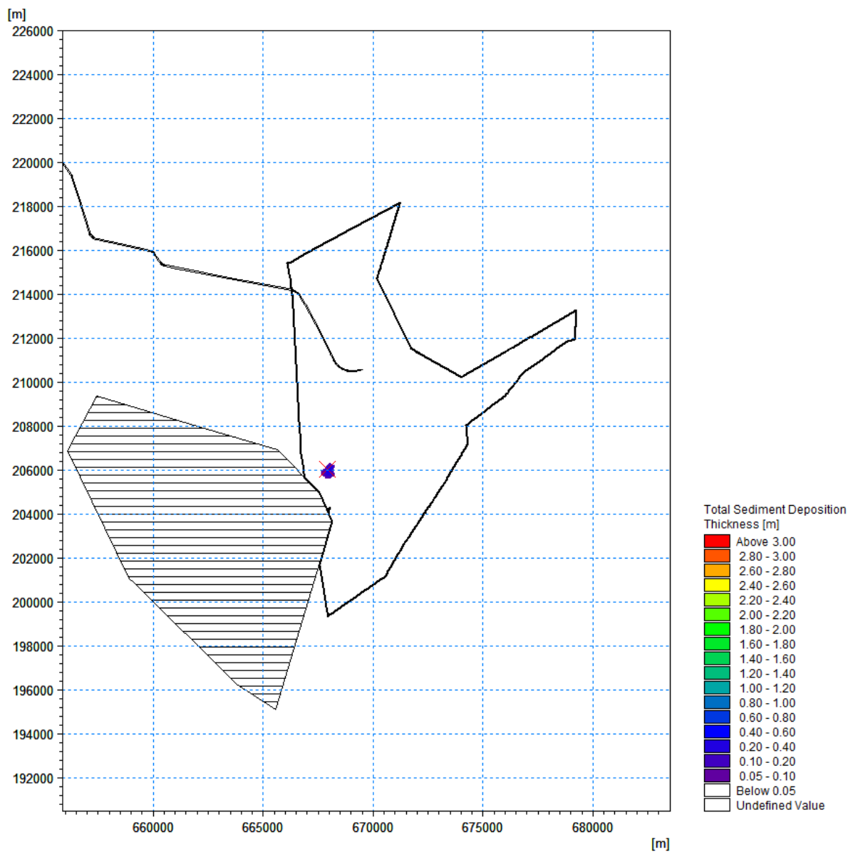
Figure 7.115 Total deposition thickness during sediment disposal - Slack water near low water during neap tide ('Zone 1 & 3' material)
