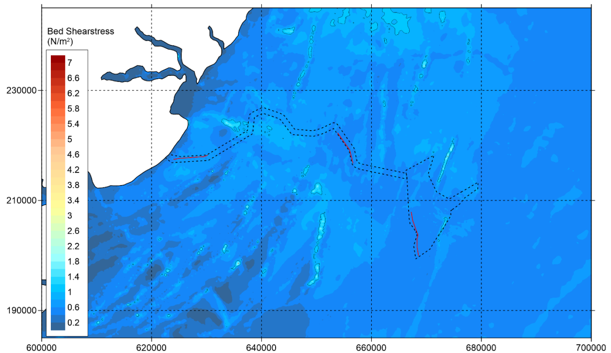
Figure 5.55 ‘Additional’ layout - Bed shear stress during neap tide - peak flood (zoomed in).
