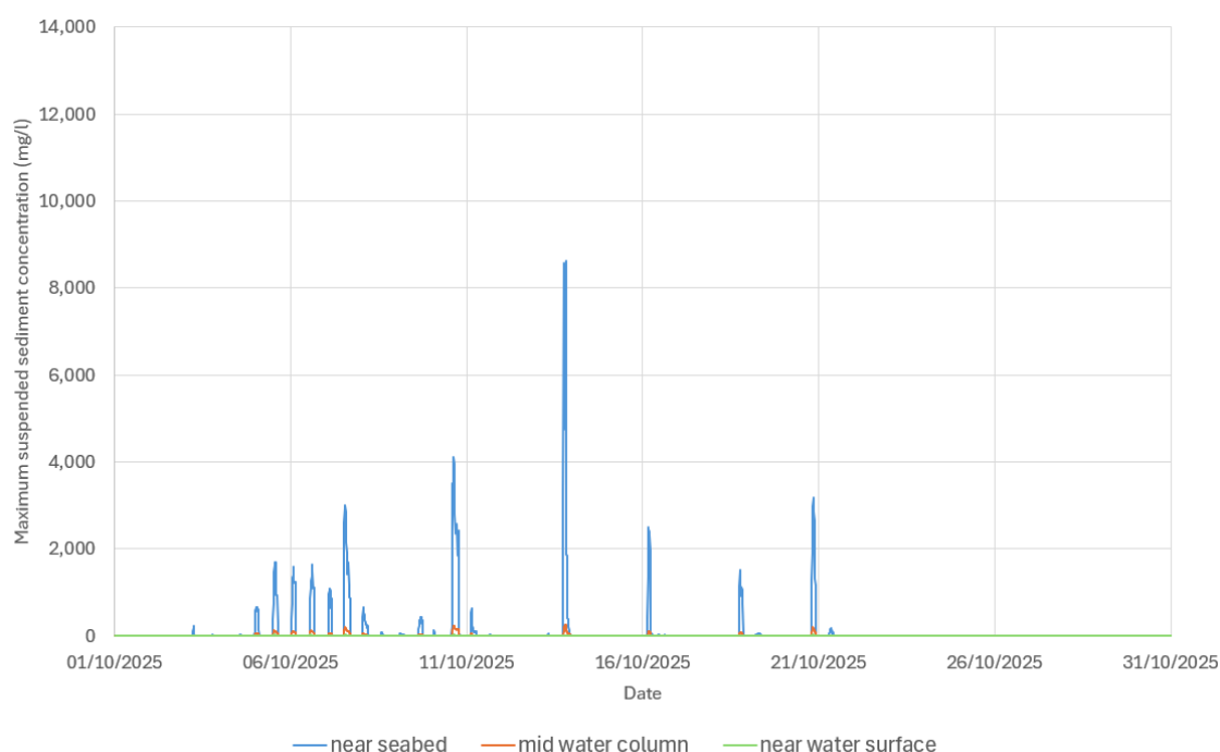
Figure 7.140 Time series of suspended sediment concentration at P4 during indicative offshore export cable levelling (including additional length), array cable levelling and seabed preparation operations for smaller WTGs layout structures for seabed, middle of water column and near water surface (array centre)
