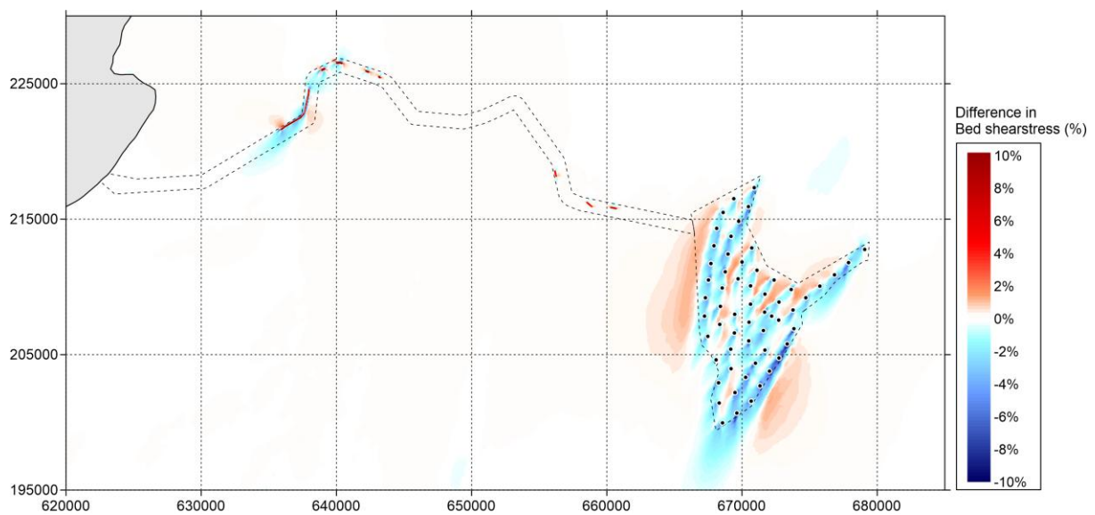
Figure 5.67 Difference in bed shear stress (in percent) between 'Baseline' and 'Option' during spring tide (positive means increase of bed shear stress by option and vice versa) – peak flood
