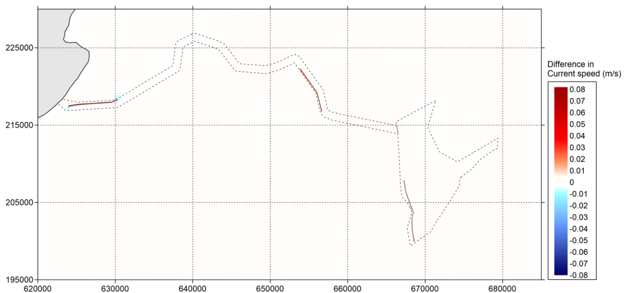
Figure 5.90 Difference in current speed (in metres/second) between 'Baseline' and 'Additional Layout' during spring tide (positive means increase of current speed by option and vice versa) – peak ebb
