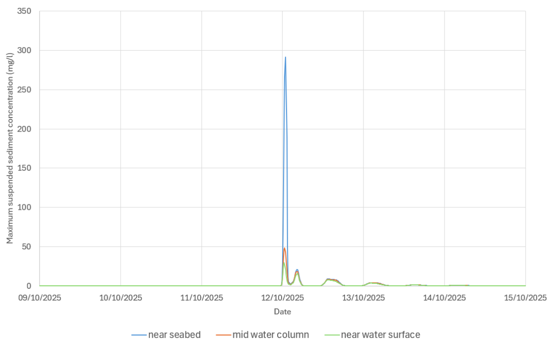
Figure 7.132 Time series of suspended sediment concentration at P1 during indicative offshore export cable levelling (including additional length) for seabed, middle of water column and near water surface (inside KKE MCZ)
