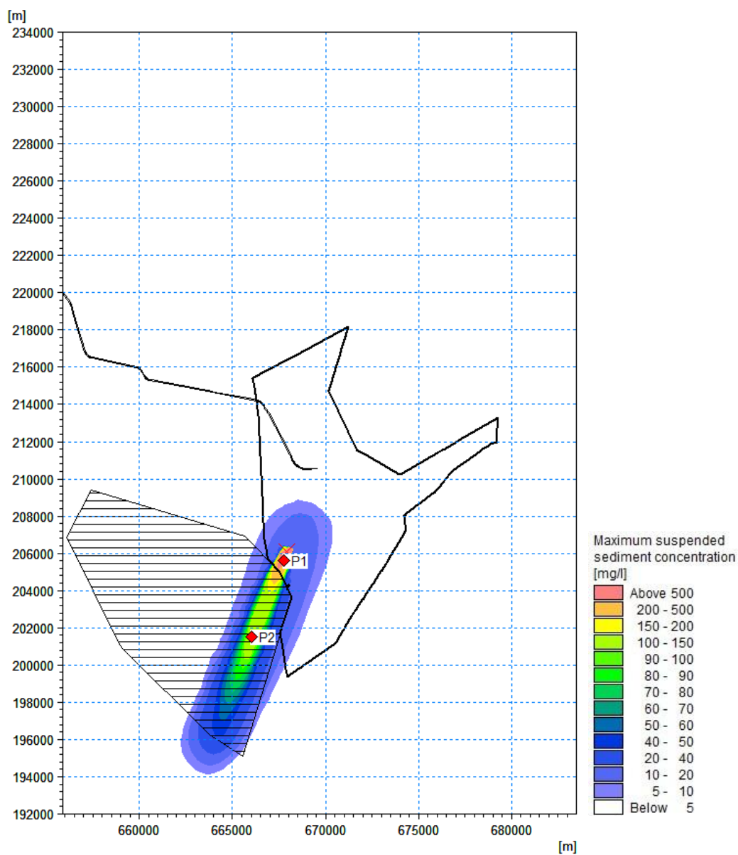
Figure 7.110 Maximum suspended sediment concentration during array disposal occurring near the seabed – Slack water near low water during neap tide ('Zone 1 & 3' material) (red point = time series extraction point)
