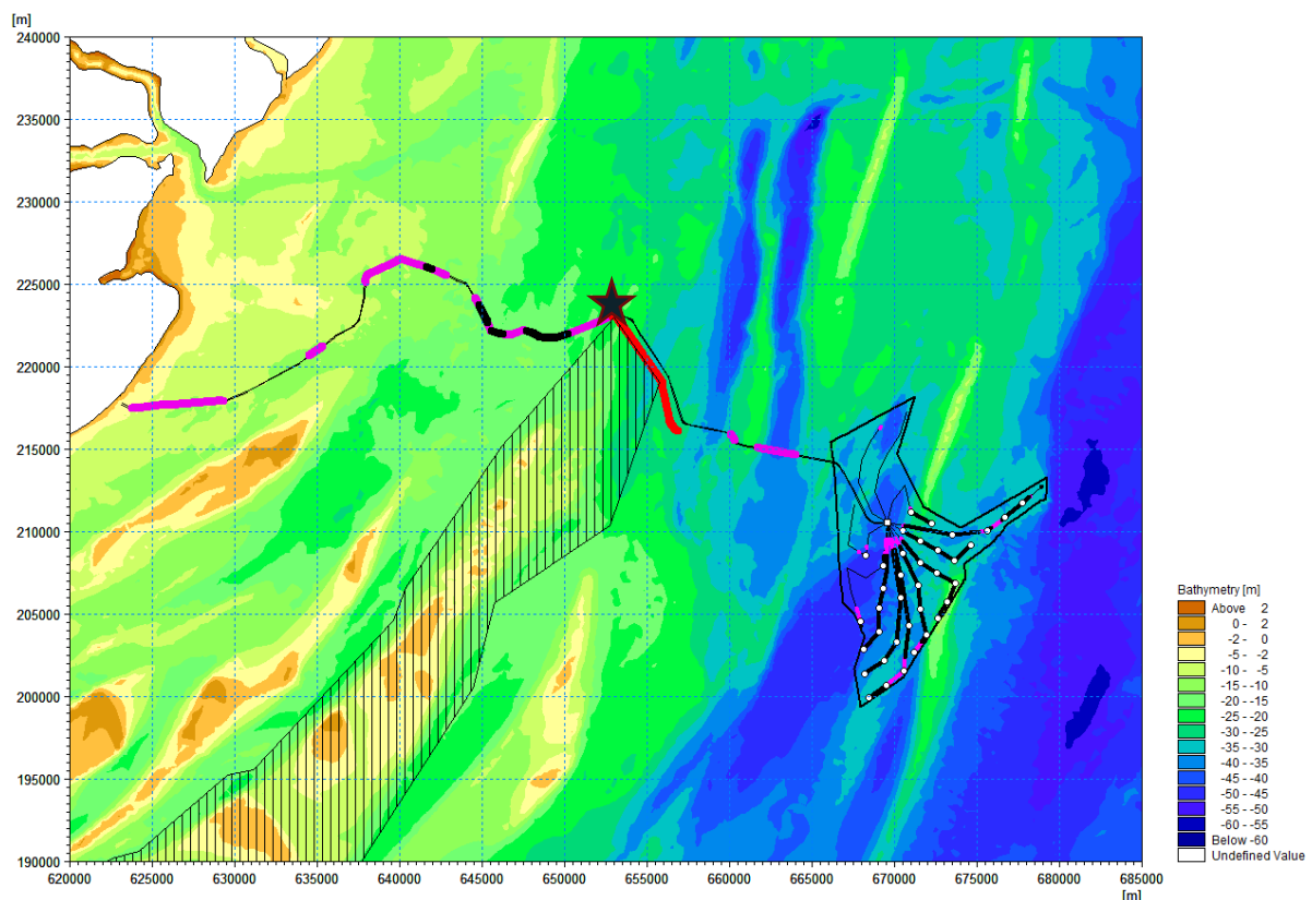
Figure 6.18 Shows the offshore export cable (including additional length) and array cable levelling; where areas through megaripples are shown as thick purple lines and areas through sandwaves are shown as thick black lines. The additional levelling length is shown as thick red
