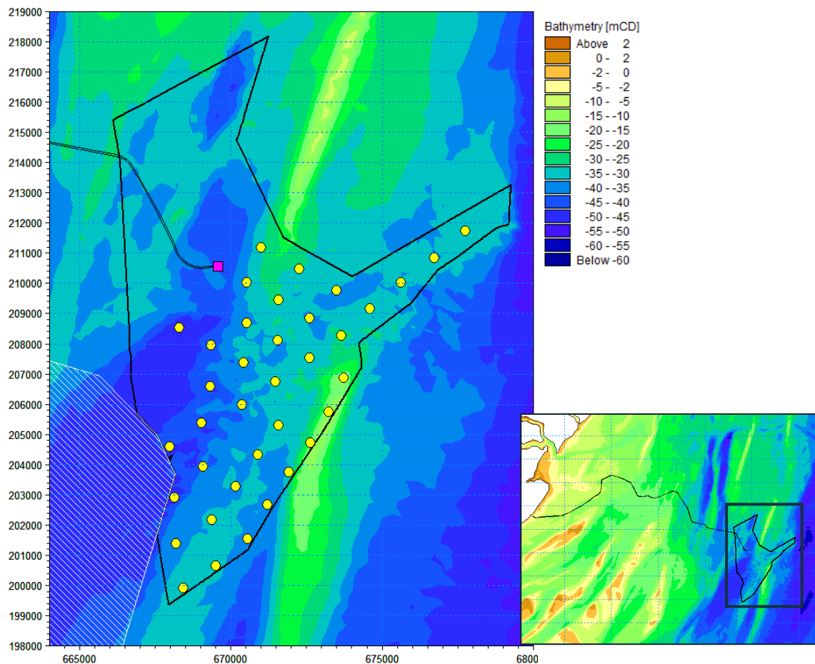
Figure 6.8 Location of seabed preparation activities for array structures – smaller WTGs indicative Layout (purple square = OCP/OSP, yellow dot = WTGs, white hatch = MCZ)
