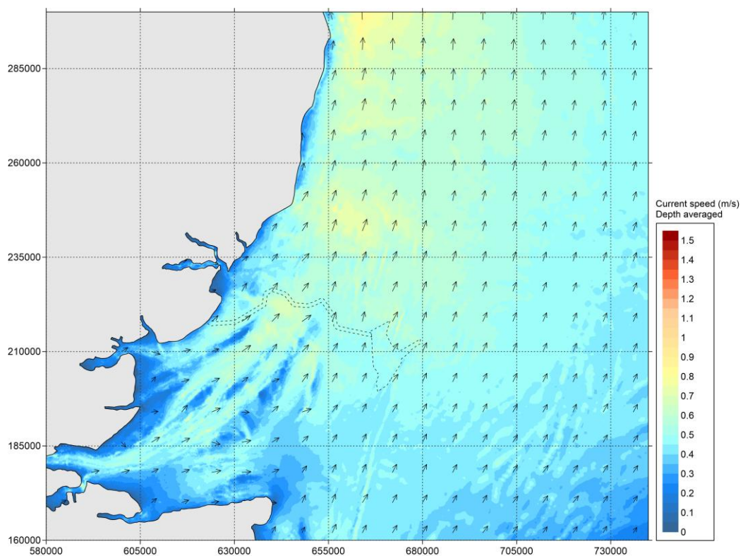
Figure 5.28 Baseline - Current speed during neap tide - peak ebb (zoomed out).
