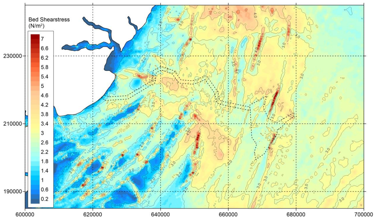
Figure 5.37 Baseline – Bed shear stress during spring tide - peak flood (zoomed in).
