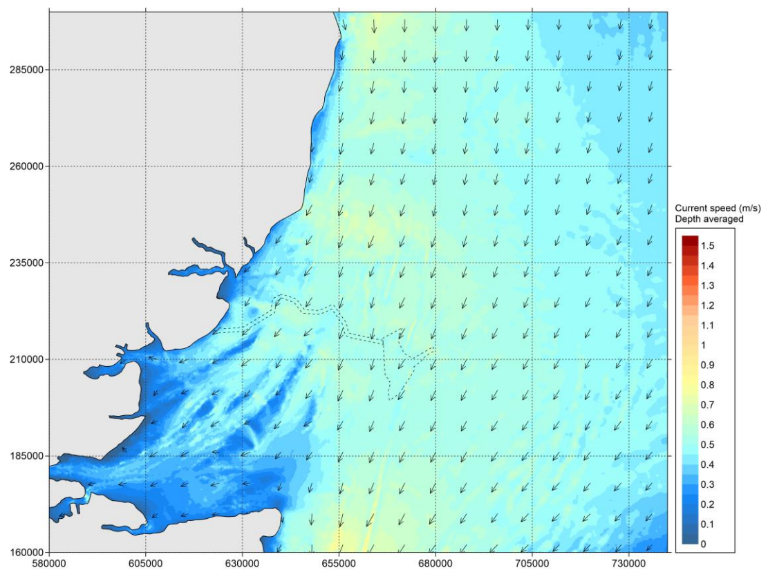
Figure 5.26 Baseline - Current speed during neap tide - peak flood (zoomed out).
