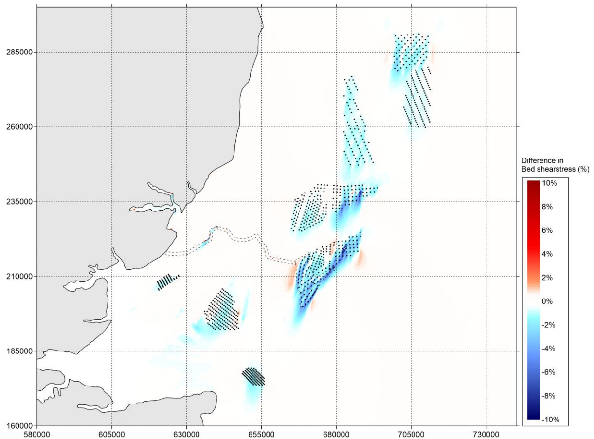
Figure 5.83 Difference in bed shear stress (in percent) between 'Baseline' and 'Cumulative' during spring tide (positive means increase of bed shear stress by option and vice versa) – peak flood
