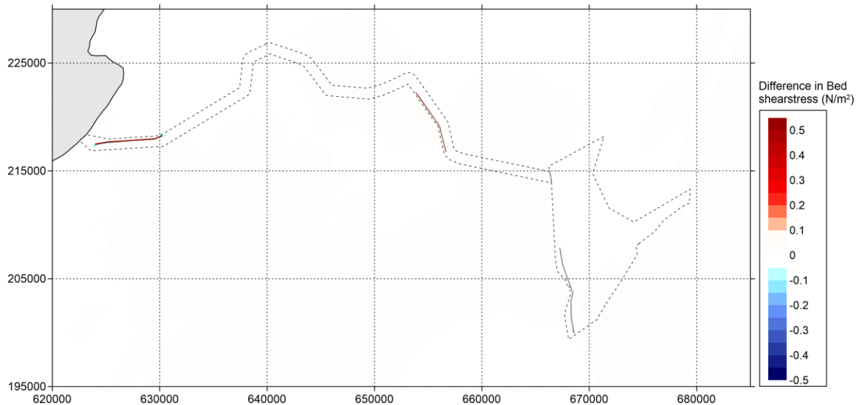
Figure 5.98 Difference in bed shear stress (in \text{N/m}^2 ) between 'Baseline' and 'Additional Layout' during spring tide (positive means increase of bed shear stress by option and vice versa) – peak ebb
