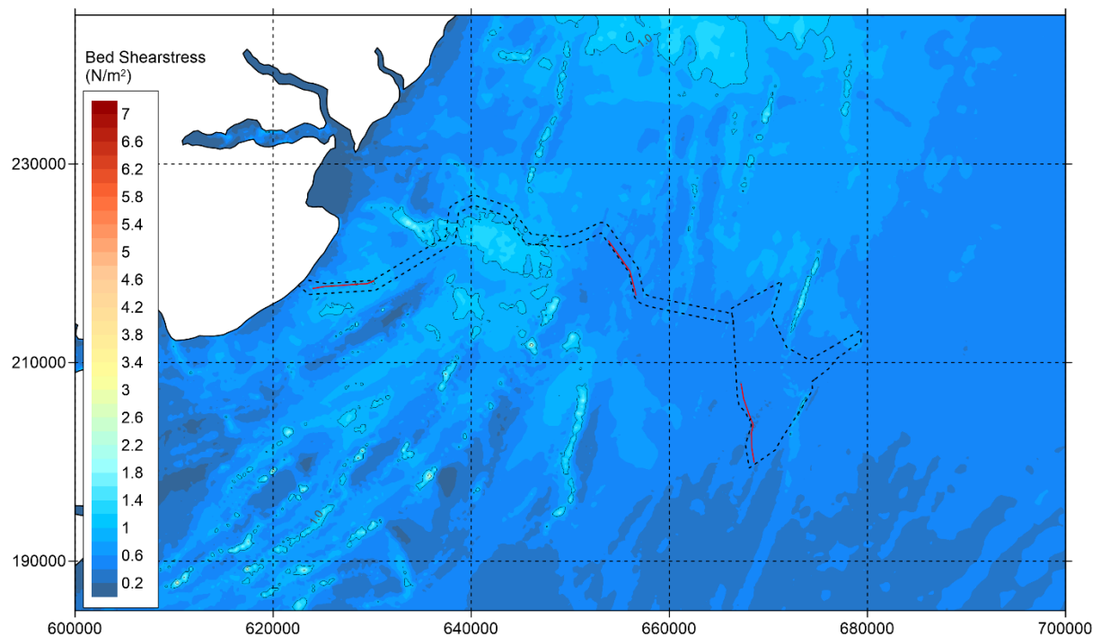
Figure 5.56 ‘Additional’ layout - Bed shear stress during neap tide - peak ebb (zoomed in).
