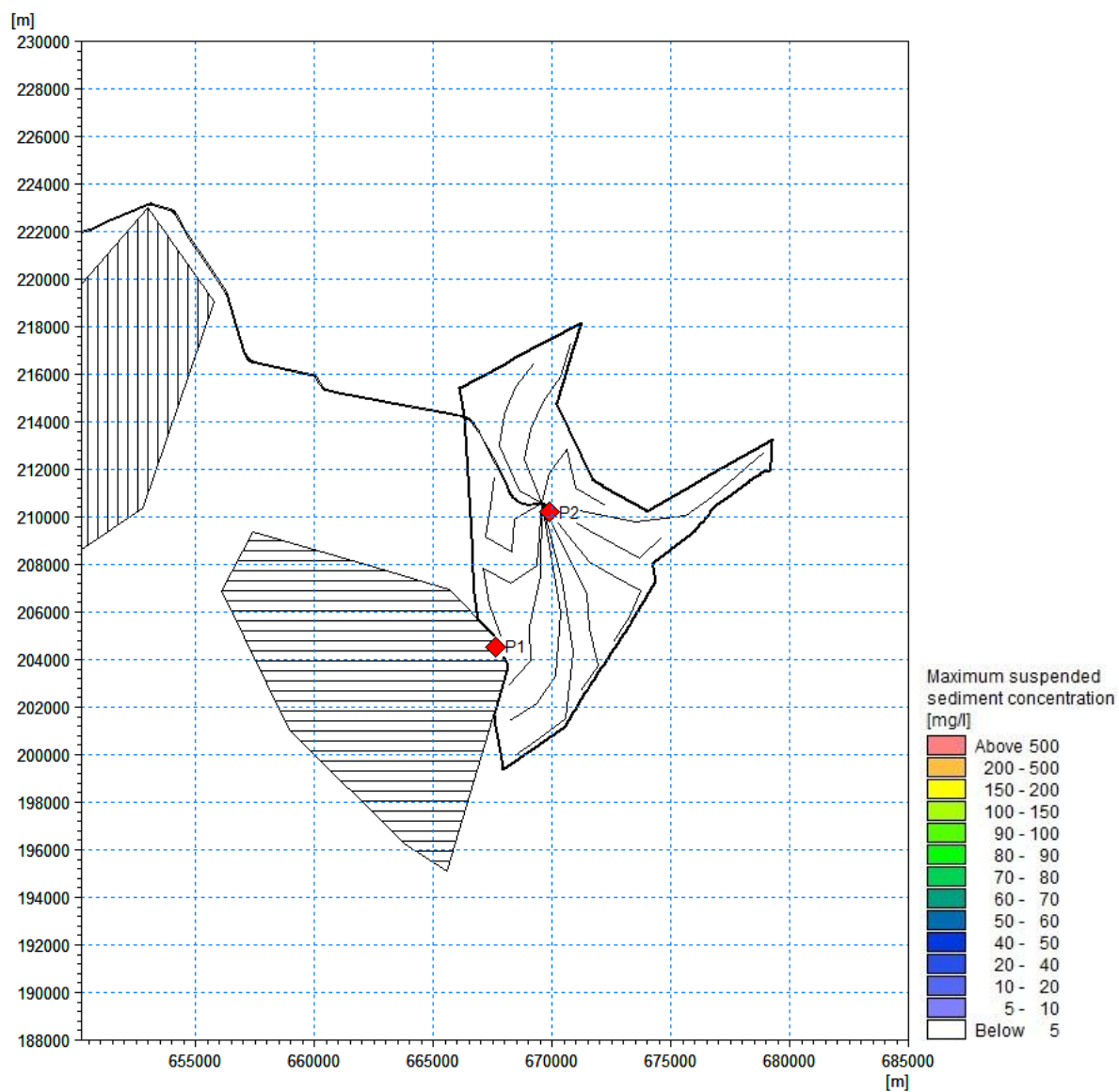
Figure 7.51 Maximum suspended sediment concentration during array cable trenching operations occurring near the water surface (red points = time series extraction points, vertical hashed area = MLS SAC, horizontal hashed area = KKE MCZ)
