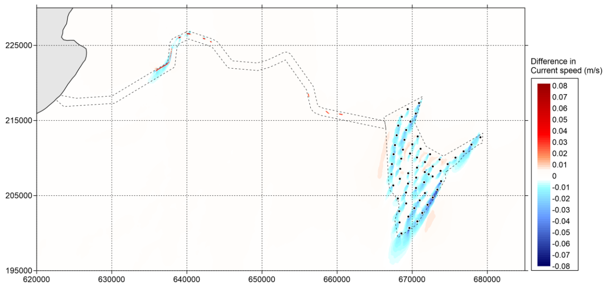
Figure 5.57 Difference in current speed (in metres/second) between 'Baseline' and 'Option' during spring tide (positive means increase of current speed by option and vice versa) – peak flood
