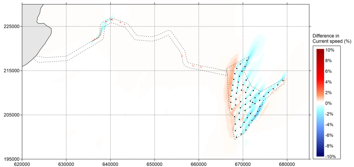
Figure 5.60 Difference in current speed (in percent) between 'Baseline' and 'Option' during spring tide (positive means increase of current speed by option and vice versa) – peak ebb
