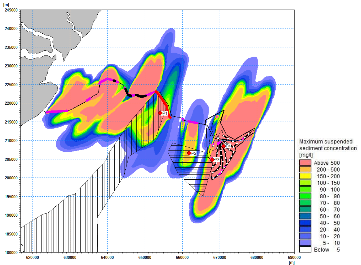
Figure 7.134 Maximum suspended sediment concentration during an indicative offshore export cable levelling (including additional length), array cable levelling and seabed preparation operations for smaller WTGs layout structures occurring near the seabed (thick purple line = MR, thick black line = SW, white points = WTG structures, red points = time series extraction points, vertical hashed area = MLS SAC, horizontal hashed area = KKE MCZ)
