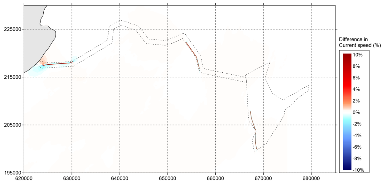
Figure 5.91 Difference in current speed (in percent) between 'Baseline' and 'Additional Layout' during spring tide (positive means increase of current speed by option and vice versa) – peak flood
