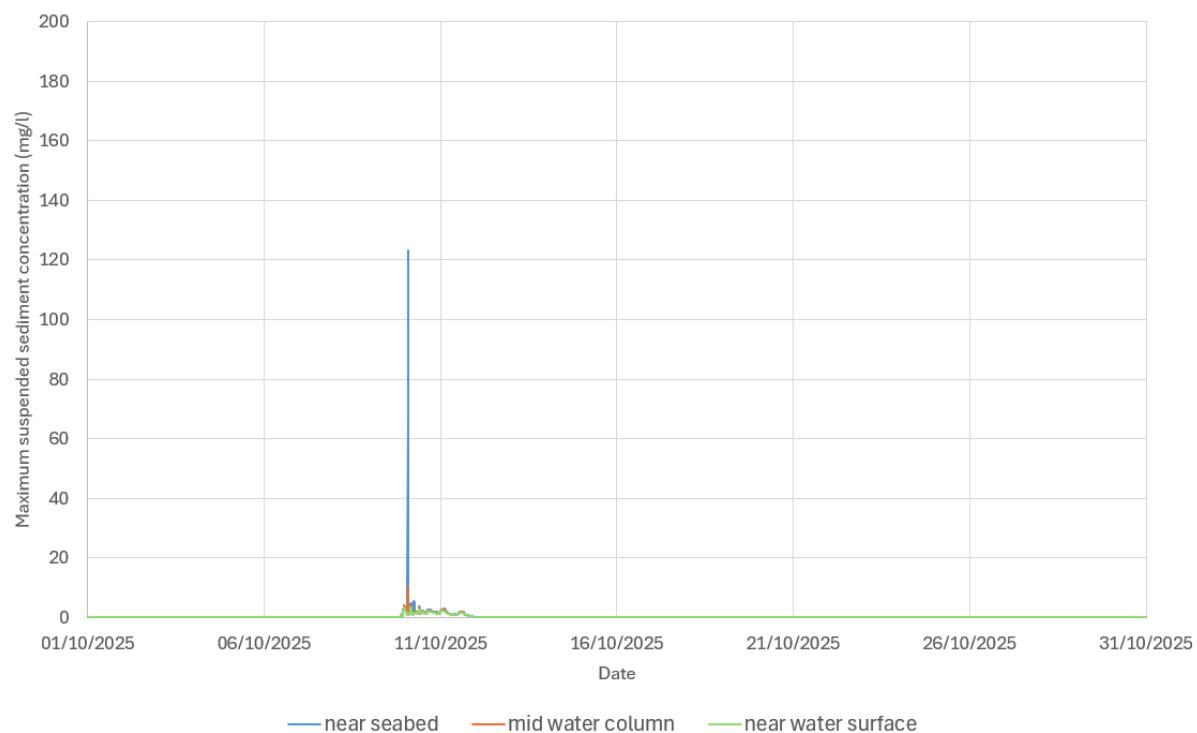
Figure 7.35 Time series of suspended sediment concentration at P2 during seabed preparation for array structures (smaller WTGs) near seabed, middle of water column and near water surface (array centre)
