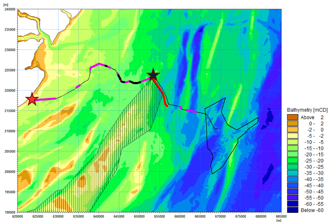
Figure 6.17 Shows where the offshore export cable levelling (including additional length) is expected to be required; where areas through megaripples are shown as thick purple lines and areas through sandwaves are shown as thick black lines. The additional levelling length is shown as thick red line. Red star indicates approximate start of export cable levelling. Black star indicates approximate start of additional levelling length.
