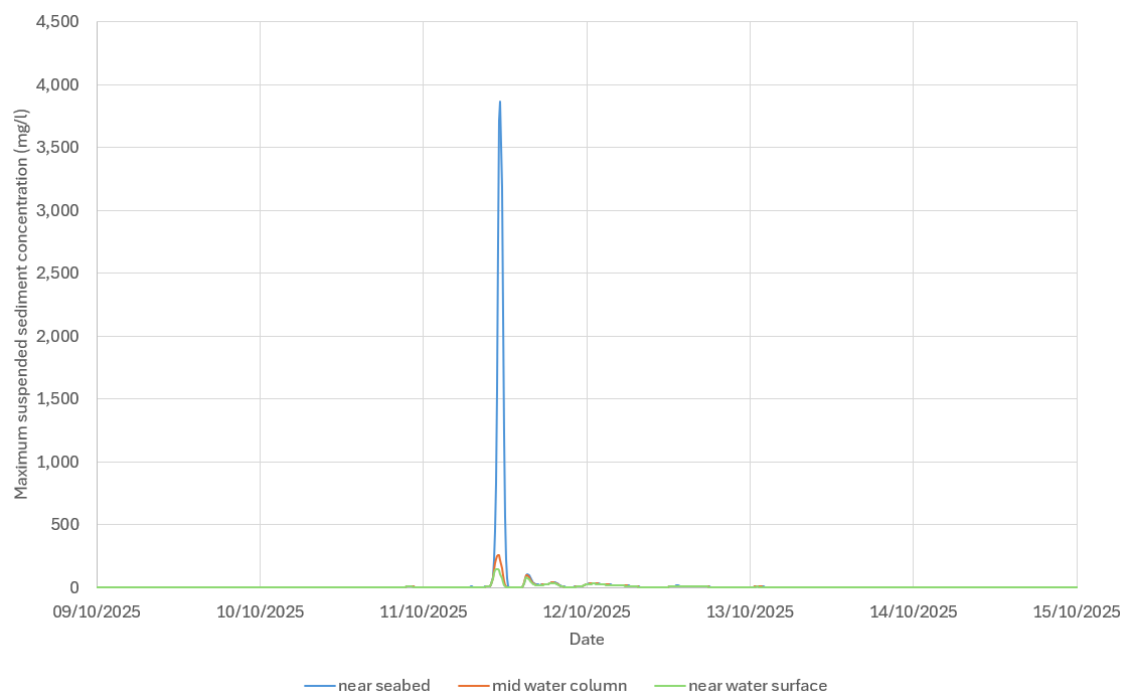
Figure 7.131 Time series of suspended sediment concentration at P1 during indicative offshore export cable levelling (including additional length) for seabed, middle of water column and near water surface (inside MLS SAC)
